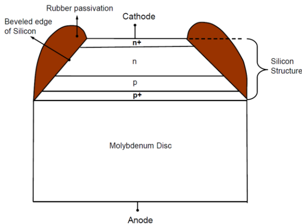
Fig. 2 – Structure of semiconductor diode
