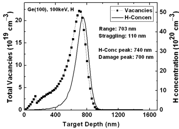
Fig. 2 – Depth profile of the implanted ions and number of vacancies produced for the energy of 100 keV hydrogen in Ge. The fluence of hydrogen ions was 1 \times 10^{17} \text{ cm}^{-2} . These simulations are done using SRIM 2008 [14]
