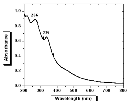
Fig. 6 – Optical absorption of pure Modified Fullerene film spin-coated from chloroform
