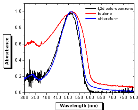
Fig. 2 – The UV-vis spectra of pure MEH-PPV film spin-coated from 1,2-dichlorobenzene, toluene and chloroform
