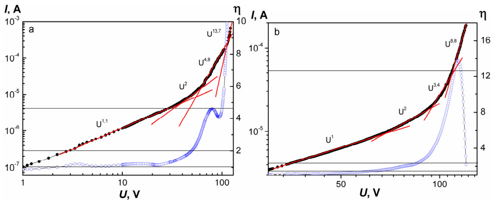
Figure 3. Double-log SCLC CVC of multilayered structures Mo/CdTe/Ag and results of their differentiation. CdTe films are prepared at T_c = 893 K and various T_s : 723 K (a); 823 K (b)
