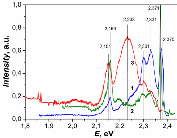
Figure 6. Photoluminescence spectra registered at T=4.5 K for ZnTe films prepared at T_s = 973 K and various T_s , K: 573 K (1); 673 K (2); 773 K (3)
