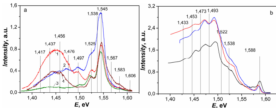
Figure 5. PL spectra registered at T=4,5 K for polycrystalline films CdTe/glass (a), prepared at T_e = 893 K and various T_s , K: 473 K (1); 523 K (2); 623 K (3); 823 K (4) and for the epitaxial layer CdTe/BaF 2 (b): T_e = 893 K, T_s = 798 K
