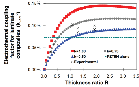
Figure 8. Electrothermal coupling factor for laminate composites ( k_{Lam}^2 ) evaluated for PZT5H-St pairs and the samples from the experiment in our previous publications[4, 5] (with k=1 interfacial factor).
