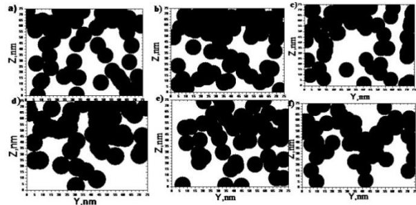
Fig. 2 – Percolation clusters induced by irradiation at different angles: a) 25 °, b) 30 °, c) 45 ° d) 60 ° e) 70 ° f) 90 °
