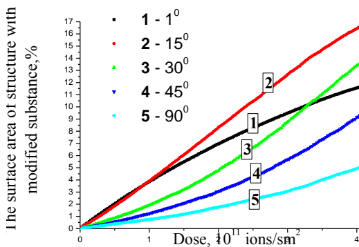
Fig. 4 – Dependence of the branched structure surface area on the dose and from different angles, irradiation of one surface
