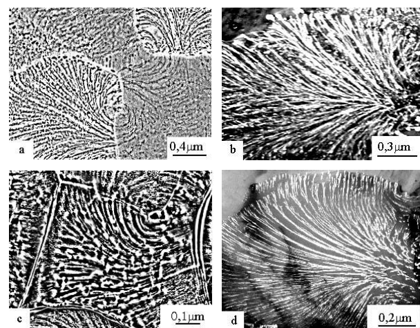
Fig. 2 – The types of crystallized structures of alloys produced by melt-spinning from 1000 °C: "Vortex" structure a) Al-0.67 at. % Sc; c) Al-0.33 at. % Zr; "Fan" structure b) Al-0.67 at. % Sc; d) Al-0.33 at. % Zr
