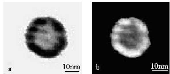
Fig. 5 – The morphology of \text{Al}_3\text{Zr}/\text{Al}_3\text{Sc} phase precipitate: a – bright-field image, b – dark-field image in superstructural reflex (100)
