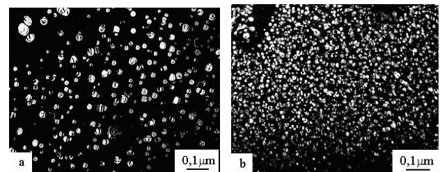
Fig. 6 – The dark-field image in superstructural reflex (110) of the \text{Al}_3\text{X} phase of the alloys: a) Al – 0.6 at. % Sc, quenching from 1400 °C at V_L = 44 m/s, aging at 450 °C for 2 hours; b) Al – 0.6 at. % Sc – 0.24 at. % Zr, quenching from 1000 °C at V_L = 44 m/s, aging at 450 °C for 40 hours
