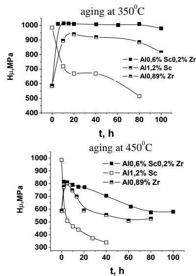
Fig. 7 – Microhardness change after isothermal aging
