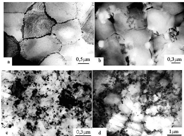
Fig. 1 – The structure of the alloys quenched from 1400 °C: a) Al-0.67 at. % Sc; b) Al-0.33 at. % Zr; c) Al-1.2 at. % Zr; d) Al-0.6 at. % Sc-0.24 at. % Zr
