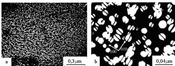
Fig. 4 – The structure of the Al – 0.89 at. % Zr alloy quenched from 1000 °C at V_L = 44 m/s and aged at 450 °C for 60 hours
