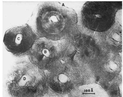
Fig. 2 – Electron-microscopic picture of a cross section of chrysotile fibers [5]
