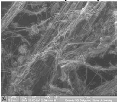
Fig. 1 – View of Bazhenov fiber commercial chrysotile P-3-60
