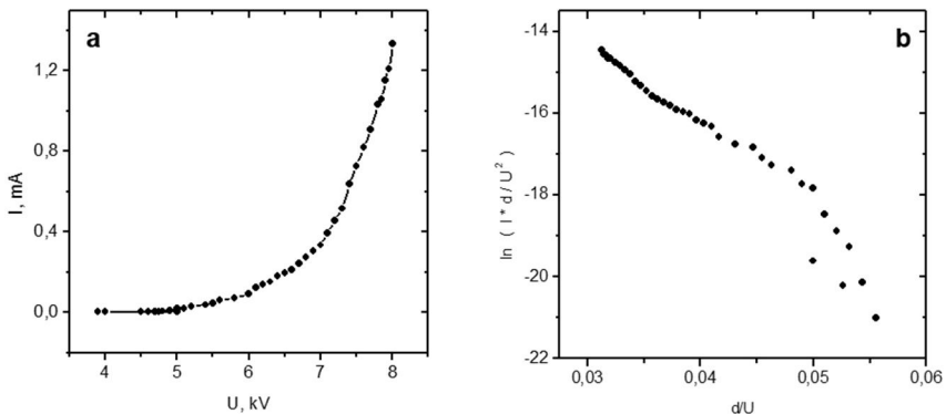
Fig. 2 a) - A voltage-current characteristic of \text{Cu-C}_{60} nanocomposite field emitter at 300 \mu\text{m} anode-cathode distance; b) - the Fowler-Nordheim plot of a voltage-current characteristic of \text{Cu-C}_{60} nanocomposite field emitter.
