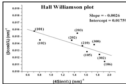
Fig. 3 – Hall-Williamson plot for ZnSe nanocrystallite
