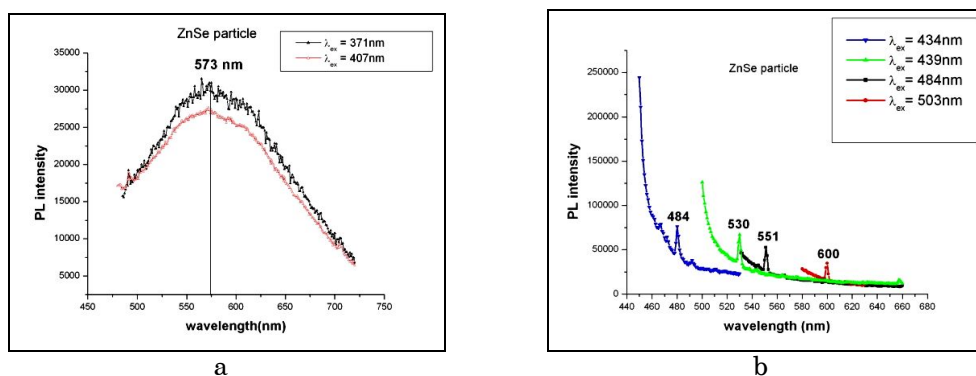
Fig. 8 – (a) and (b) shows PL spectra of ZnSe nanoparticles
