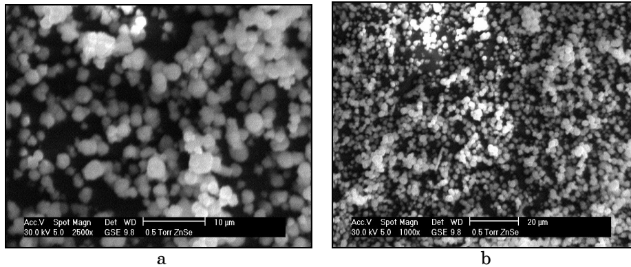
Fig. 7 – SEM micrograph of ZnSe nanoparticles
