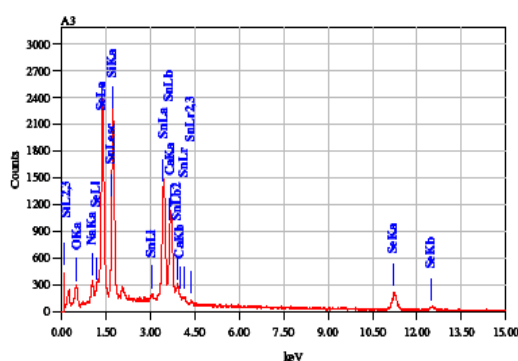
Fig. 3 – EDAX Spectra of SnSe thin film (100 nm) deposited at room temperature on the glass substrate
