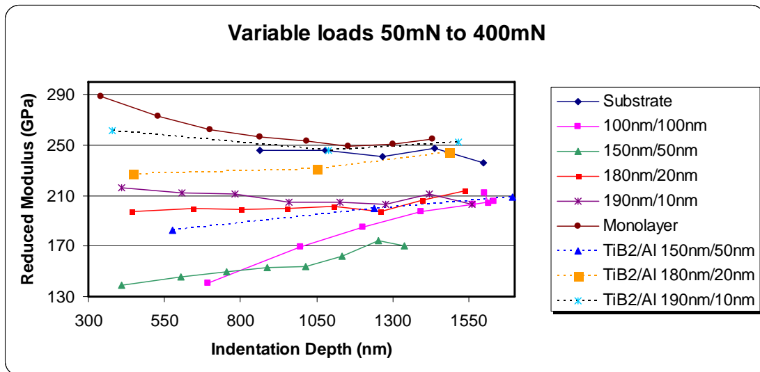
Figure 3: The variation in Reduced Modulus as a function of indent depth on multilayers of TiB 2 /C. The captions in the figure show the thicknesses of the TiB 2 /C layers. In all cases, a total film thickness of 5 μm was produced and the volume fraction of TiB 2 ceramic was altered by changing the TiB 2 /C layer thicknesses. The data for the substrate and a monolayer of TiB 2 is also plotted. The data from Cruz [19] for a similar TiB 2 /Al stack is plotted for comparison.
