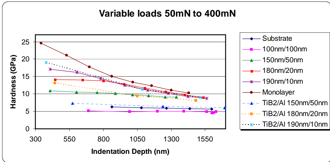
Figure 2: The variation of the hardness as a function of indentation depth for variable loads on multilayers of TiB 2 /C. The captions in the figure show the thicknesses of the TiB 2 /C layers. In all cases, a total film thickness of 5 μm was produced and the volume fraction of TiB 2 ceramic was altered by changing the TiB 2 /C layer thicknesses'. The data for the substrate and a monolayer of TiB 2 is also plotted. The data from Cruz [19] for a similar TiB 2 /Al stack is plotted for comparison.
