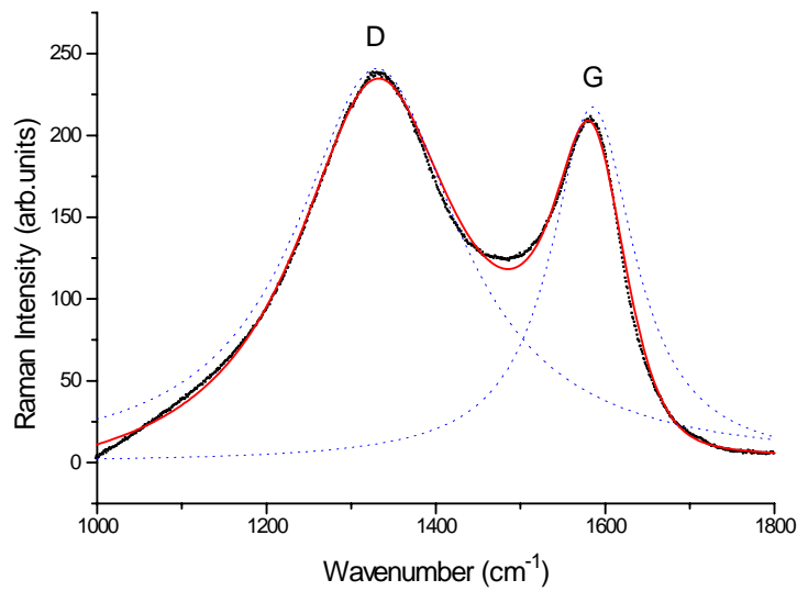
Figure 1: Raman spectra from the carbon film fabricated in this study. Lorentzian fits (only two are shown) at 1360 and 1580 \text{cm}^{-1} were used to fit the positions of the D and G peaks. Additional peaks at 1170 and 1500 \text{cm}^{-1} were necessary to accurately fit the data. Additional peaks in the Raman spectra around 1100-1220 \text{cm}^{-1} have been associated with hexagonal diamond [17,16]. The Raman peak at 1500 \text{cm}^{-1} has been attributed to the semicircle stretching of carbon atoms in single aromatic rings [18].
