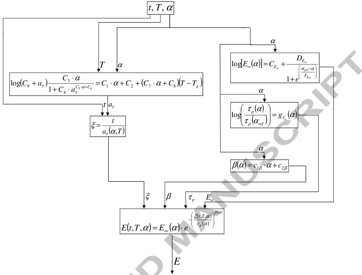
Figure 8 – Sub-model schematic.
