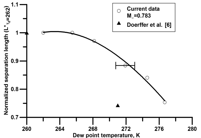
Fig. 10 Shock-induced separation length as a function of dew point temperature.
