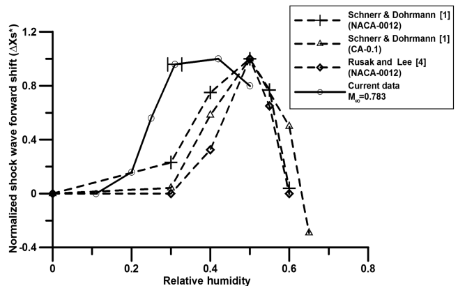
Fig. 8 Main forward shock wave shift as a function of relative humidity.
