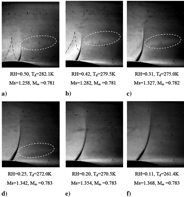
Fig. 5 Schlieren images of shock waves over bump model, M_\infty = 0.781-0.783 .
