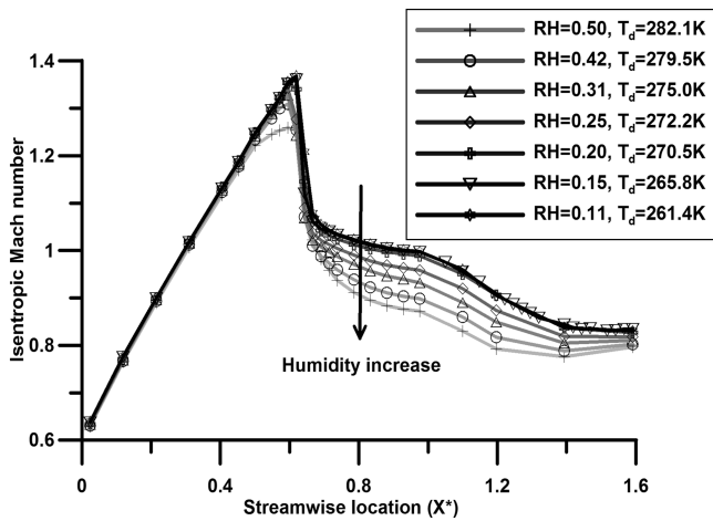
Fig. 6 Mach number distribution over the bump, M_\infty = 0.781-0.783 .
