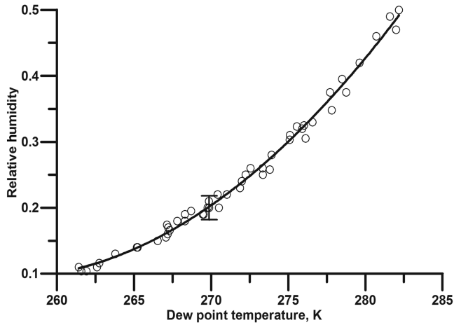
Fig. 2 Relative humidity versus dew point temperature for the wind-tunnel inlet.
