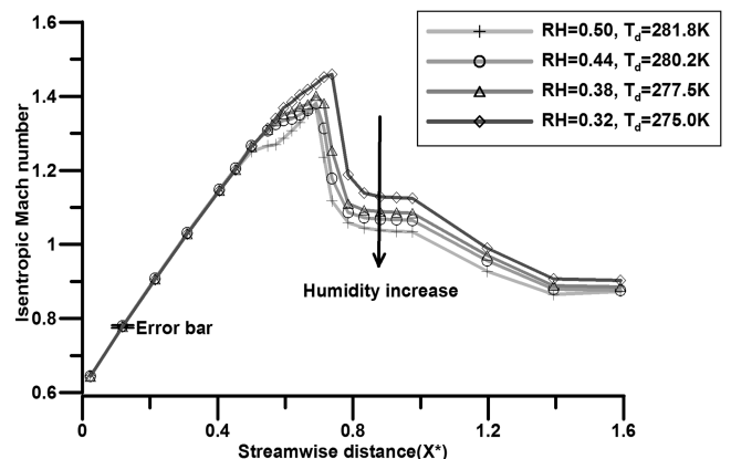
Fig. 4 Mach number distribution over the bump, M_\infty = 0.800\text{--}0.805 .
