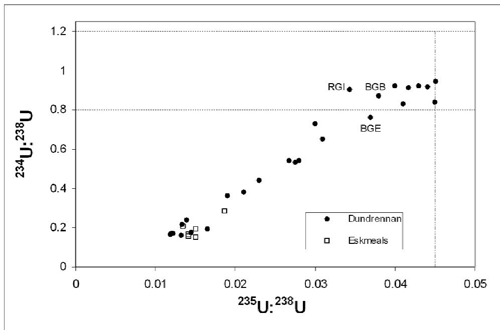
Figure 6: ^{235}\text{U}:^{238}\text{U} v ^{234}\text{U}:^{238}\text{U} ratios for Dundrennan and Eskmeals soils. The horizontal dashed lines indicate the range (upper and lower limits) of the ^{234}\text{U}:^{238}\text{U} ratio observed for natural U in soils, thus values below are indicative of DU affected soils. The vertical dashed line indicates the natural ^{235}\text{U}:^{238}\text{U} ratio, thus all values to the left identify soils as DU affected. Samples Balig Gun B (BGB), Raeberry Gun I (RGI) and Balig Gun E (BGE) indicated.
