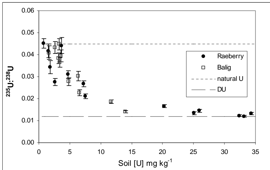
Figure 5: Soil U concentration v ^{235}\text{U}:^{238}\text{U} isotope activity ratio for Raeberry and Balig Gun soil samples. Natural and DU isotope ratio lines indicated. Error bars, where they exceed symbol margins, show uncertainties associated with tracer activity ( ^{232}\text{U} ), counting statistics, sample weighing and sample replication.
