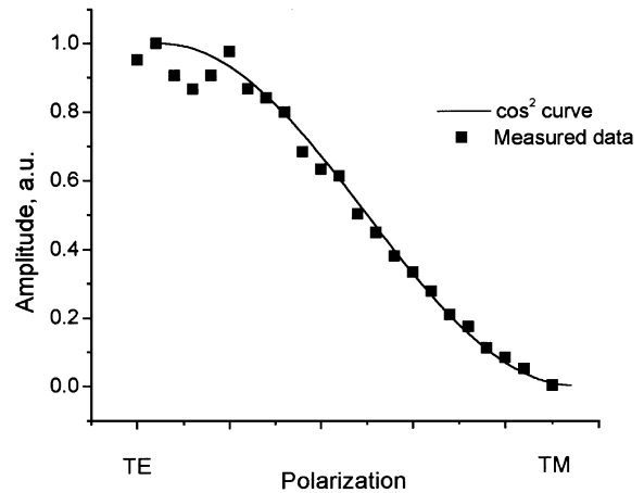
Fig. 2. Polarization dependence of the electrical signal. The solid squares are experimental points taken for different input polarization states. The signal presents \cos^2 behavior (solid curve) typical of optical rectification.
