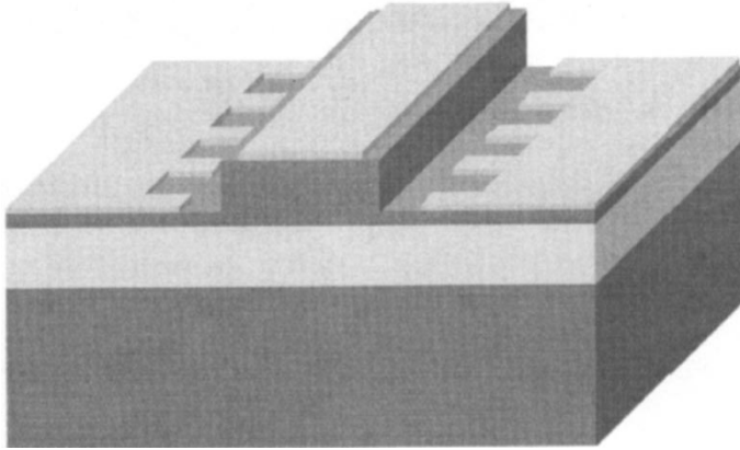
Fig. 1. Schematic of an ORE device. The central conductor of the CPW line is aligned on top of the optical waveguide. The ground electrodes are periodically loaded to create a traveling wave ORE device.
