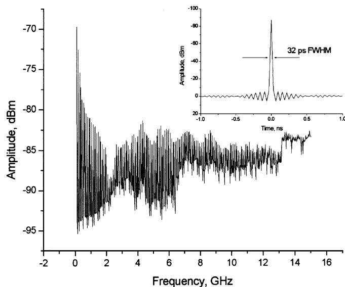
Fig. 3. Frequency spectrum of the electrical signal. The harmonics are spaced 86.7 MHz which corresponds to the repetition rate of the laser. Inset: Frequency spectrum converted into time domain by using FFT.
