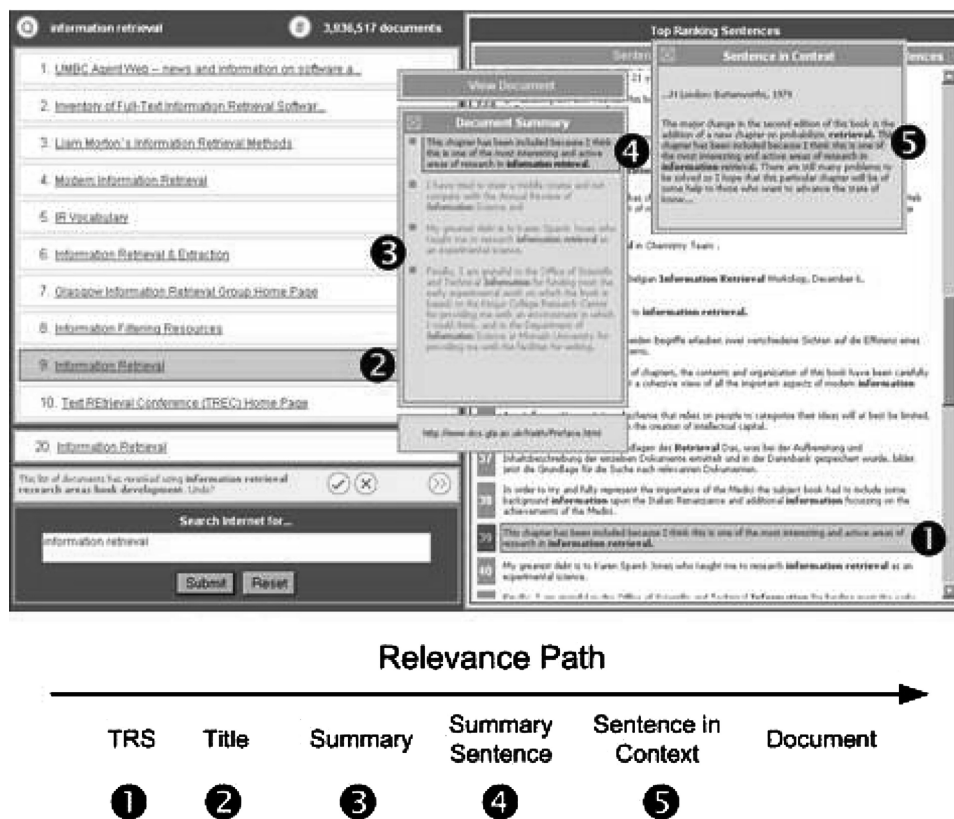
Fig. 1. Example search interface and full relevance path.
