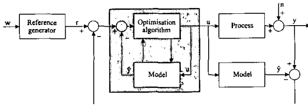
Fig. 1. Block diagram of model predictive control system
