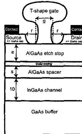
Figure 4: Cross section of PHEMT considered in this work. The distances referred to with a letter have been shrunk in the scaling process. The 10-nm InGaAs channel has an indium content of 0.2
