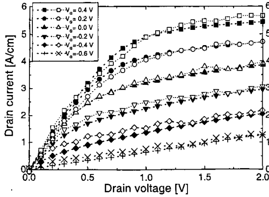
Figure 5: I_D - V_D characteristic of the PHEMT with a gate length of 120 nm. Full symbols represent experimental data for several fixed gate voltages. Open symbols are MC simulations when external resistances of the drain and source are included.
