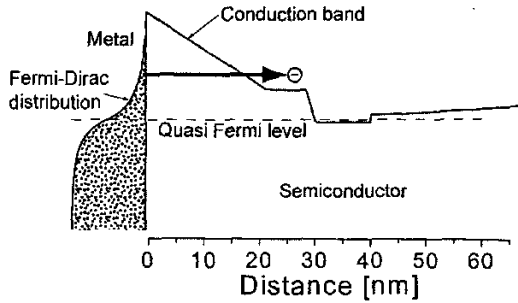
Figure 2: Cross section of the device through the middle of the gate at gate and drain biases of -1.0 and 2.0 V respectively. The simulation of tunnelling from the metal gate into the supply layer is schematically shown.
