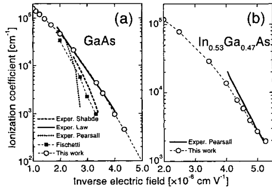
Figure 1: Impact ionisation coefficients versus inverse applied electric field obtained from simulations for GaAs (a) and for In 0.53 Ga 0.47 As (b) compared to experiments and full band simulations.
