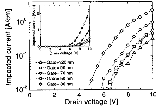
Figure 7: Impact ionisation assisted drain current versus the drain voltage at V_G = -1.0 V for the scaled PHEMTs. The inset shows the same curves on a linear scale.
