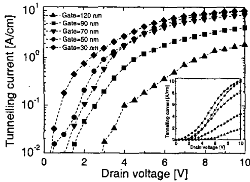
Figure 8: Tunnelling assisted drain current versus the drain voltage at V_G = -1.0 V for the scaled PHEMTs. The inset shows again the same curves on a linear scale.
