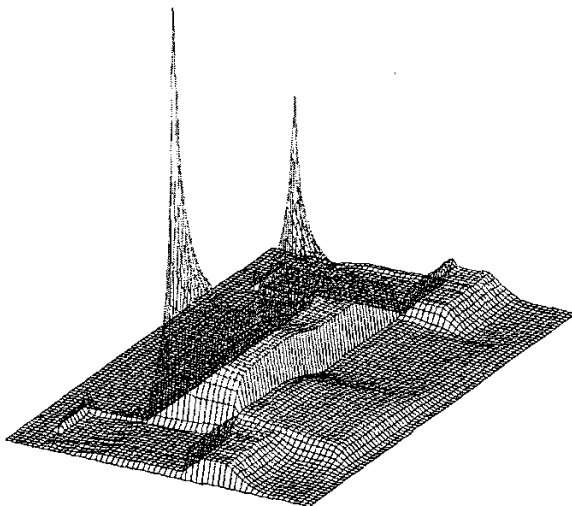
Figure 3: Electric field in the 120-nm gate length PHEMT at V_G = -1.0 V and V_D = 2.0 V. The huge electric fields which surround the gate and peak beneath the recesses determine a particle trajectory after tunnelling.
