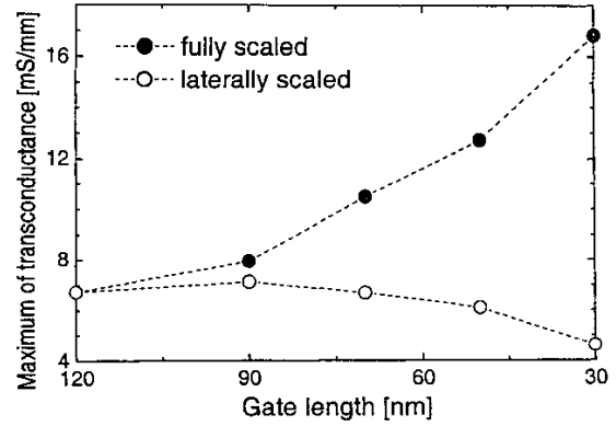
Figure 6: Maxima of transconductance as a function of the device gate lengths for fully scaled PHEMTs compared with those of laterally only scaled devices.
