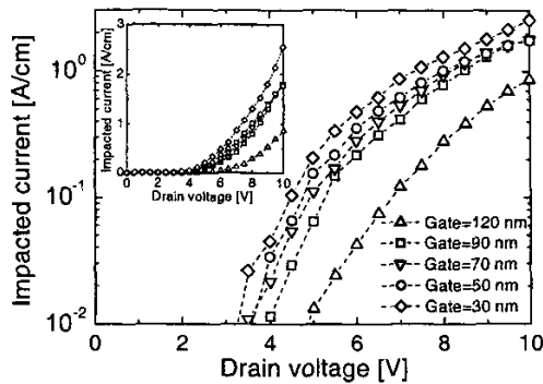
Figure 9: Impact ionisation assisted drain current versus the drain voltage at V_G = -1.0 V for the scaled PHEMTs when the tunnelling is included in the device simulations. The inset shows again the same curves on a linear scale.
