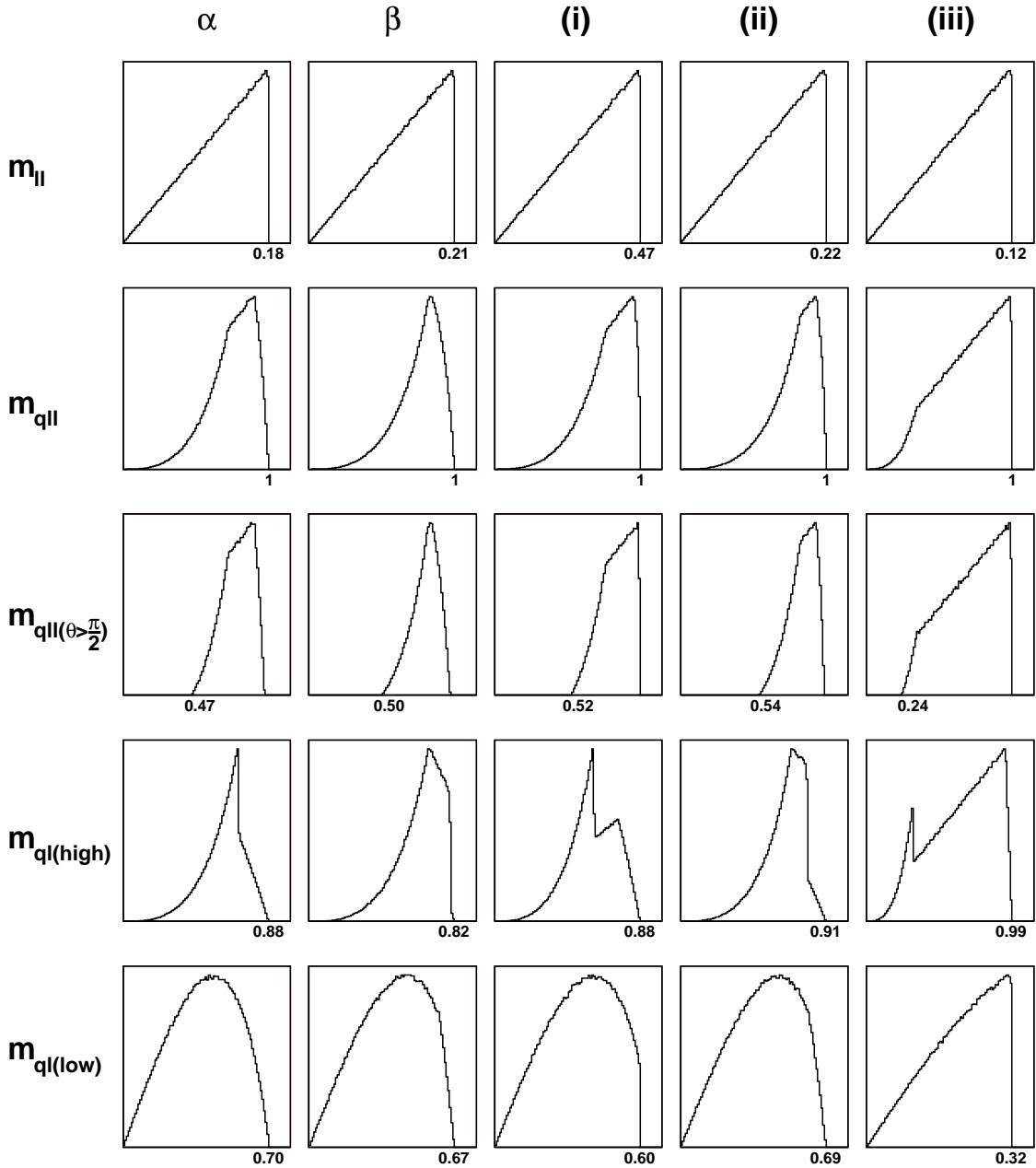
Figure 10: Theoretical mass distributions for SPS 1a ( \alpha ) and ( \beta ), as well as for three other mass scenarios, denoted (i), (ii) and (iii). Kinematic endpoints are given in units of m_{qII}^{\max} . (More details will be given in [42].)
