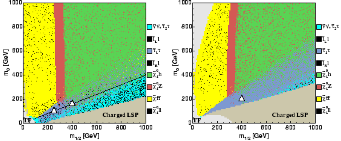
Figure 5: Decay channels of \tilde{\chi}_2^0 with A_0 = -m_0 , \tan\beta = 10 (left) and A_0 = 0 , \tan\beta = 30 (right). (See the caption of Fig. 2.)
