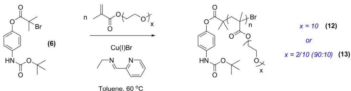
Figure 12. Polymerization of oligo(ethylene glycol) methacrylates using initiator ( 6 ) as a route to \alpha -Boc-protected polymers.
