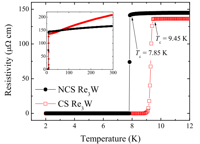
FIG. 3: (Color online) Low-temperature ac electrical resistivity of the NCS and the CS phases of \text{Re}_3\text{W} . The inset shows the electrical resistivity of both phases up to room temperature.
