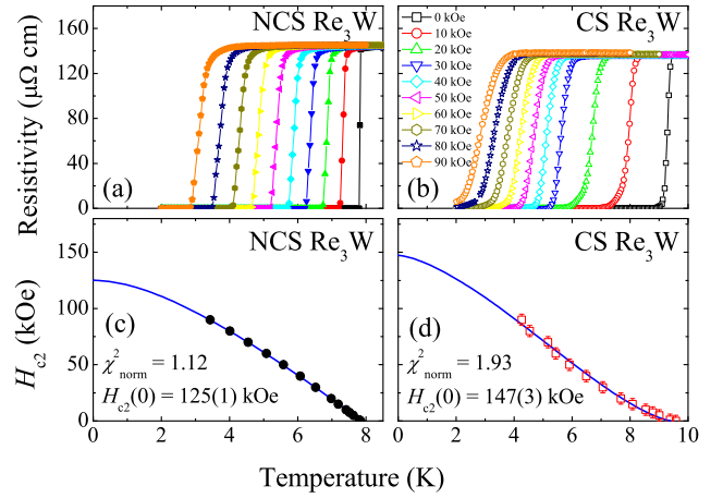
FIG. 7: (Color online) (a) and (b) Temperature variation of the resistivity in a set of magnetic fields from 0 to 90 kOe for the NCS and CS phases of \text{Re}_3\text{W} . (c) and (d) Temperature dependence of the upper critical fields of the NCS and CS phases of \text{Re}_3\text{W} . The solid line in Fig. 7(c) is a fit to the data using the WHH model. The solid line in Fig. 7(d) is a fit to the data using H_{c2}(T) = H_{c2}(0)(1 - (T/T_c)^{3/2})^{3/2} .
