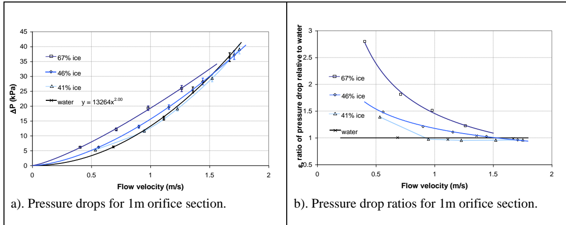
Fig. 4. Flow through a straight 1m long pipe containing an orifice at its midpoint.
