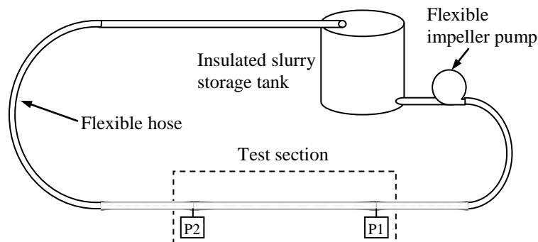
Fig. 1. Experimental set-up.
