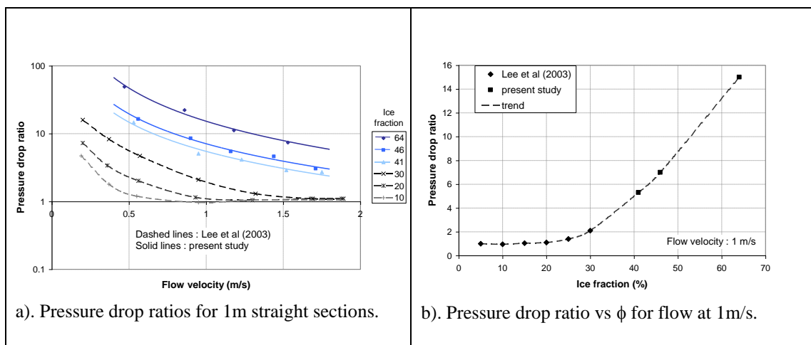
Fig. 3. Comparison of results for flow through a straight 1m long pipe.
