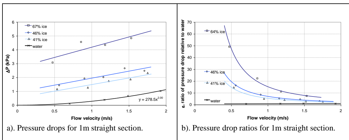
Fig. 2. Flow through a straight 1m long pipe.
