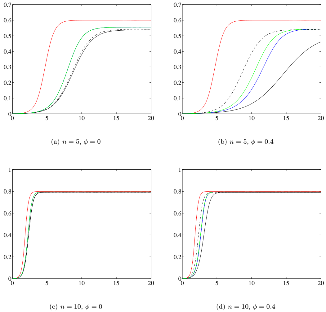
Fig. 5 Prevalence time series for networks generated using the iterative algorithm along with the results given by moment closure equations. In all plots N = 10,000 , \tau = 0.5 and \gamma = 1 with varying n and \phi . The solid black line is for simulation results from the iterative algorithm and the black dashed line is for simulation results from the same iterative algorithm but with the networks unclustered. The red line is the mean-field approximation, the blue line is the ordinary pairwise approximation (OPA) and the green line is for the improved pairwise approximation (IPA). In the cases where \phi = 0 the OPA and IPA coincide.
