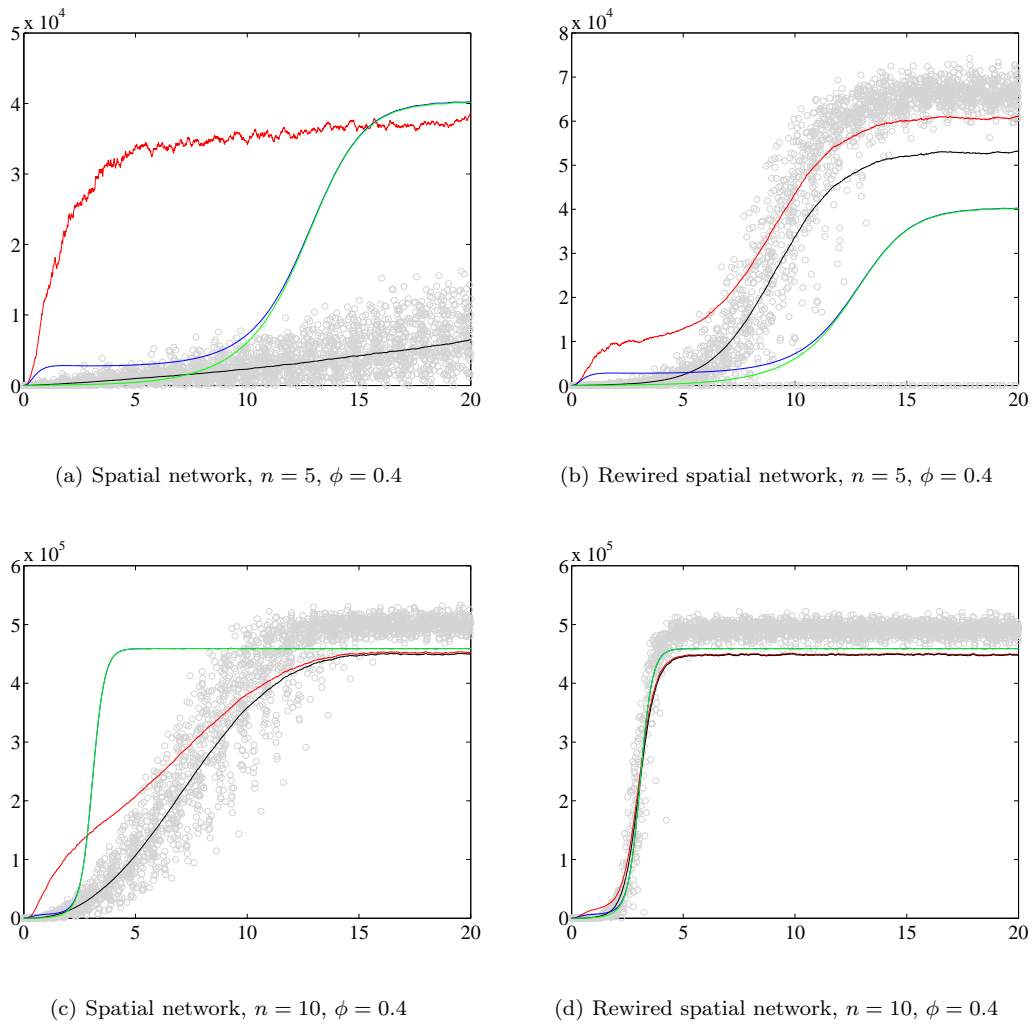
Fig. 7 Showing [III] triples counted in different ways for n = 5, 10 and \phi = 0.4 on spatial networks and their big-V rewired counterparts. The grey cloud shows actual counts of (I - I - I) triple from individual stochastic realisations. The blue and green line show [III] calculated using the OPA given by Eq. (29) and the IPA given by Eq. (28) respectively with both using pair and individual values from solving the macro ODE system (Eqs. (9 - 13)). The red and black lines show the OPA and IPA respectively, but with values for individuals and pairs as averages from the stochastic simulation.
