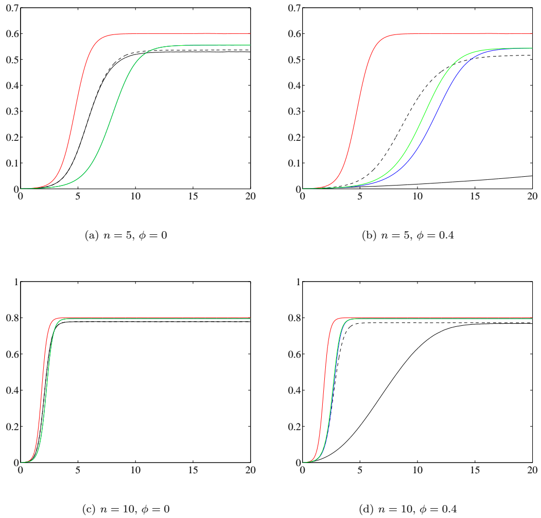
Fig. 3 Infection prevalence time series for networks generated using the spatial algorithm along with results given by moment closure equations. In all plots N = 10,000 , \tau = 0.5 and \gamma = 1 with varying n and \phi . The solid black line is for simulation results from the spatial algorithm and the black dashed line is for simulation results from the same spatial algorithm but with the networks reclustered using big-V rewiring. The red line is the mean-field approximation, the blue line is the ordinary pairwise approximation (OPA) and the green line is for the improved pairwise approximation (IPA). In the cases where \phi = 0 the OPA and IPA coincide.
