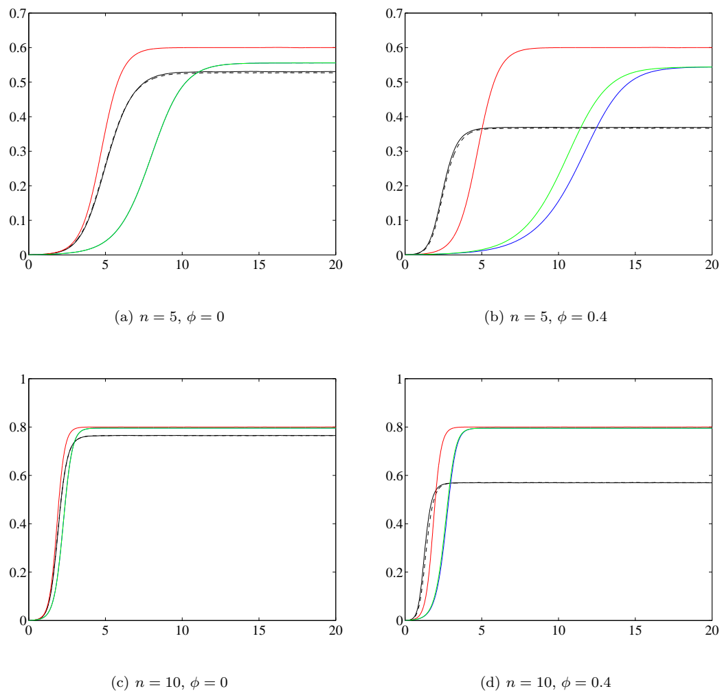
Fig. 4 Infection prevalence time series for networks generated using the group-based algorithm along with the results given by moment closure equations. In all plots N = 10,000 , \tau = 0.5 and \gamma = 1 with varying n and \phi . The solid black line is for simulation results from the group-based algorithm and the black dashed line is for simulation results from the same group-based algorithm but with the networks reclustered using big-V rewiring. The red line is the mean-field approximation, the blue line is the ordinary pairwise approximation (OPA) and the green line is for the improved pairwise approximation (IPA). In the cases where \phi = 0 the OPA and IPA coincide.
