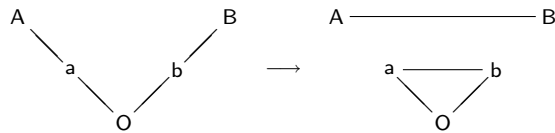
(b) Big-V rewiring
