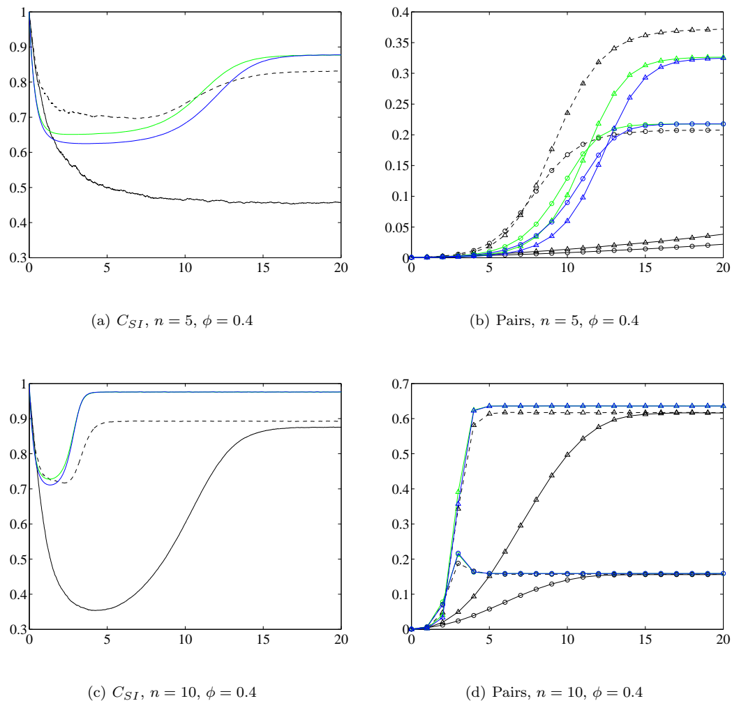
Fig. 6 Figures ?? & ?? show time series for the correlation C_{SI} as defined in Eq. (26). Figures ?? & ?? show time series for proportion of pairs that are (S, I) (circles) and (I, I) (triangles). In all plots N = 10,000 , \tau = 0.5 and \gamma = 1 . The solid black line is for simulation results from the spatial algorithm and the black dashed line is for simulation results from the same spatial algorithm but with the networks reclustered using big-V rewiring. The blue line is the ordinary pairwise approximation (OPA) and the green line is for the improved pairwise approximation (IPA).
