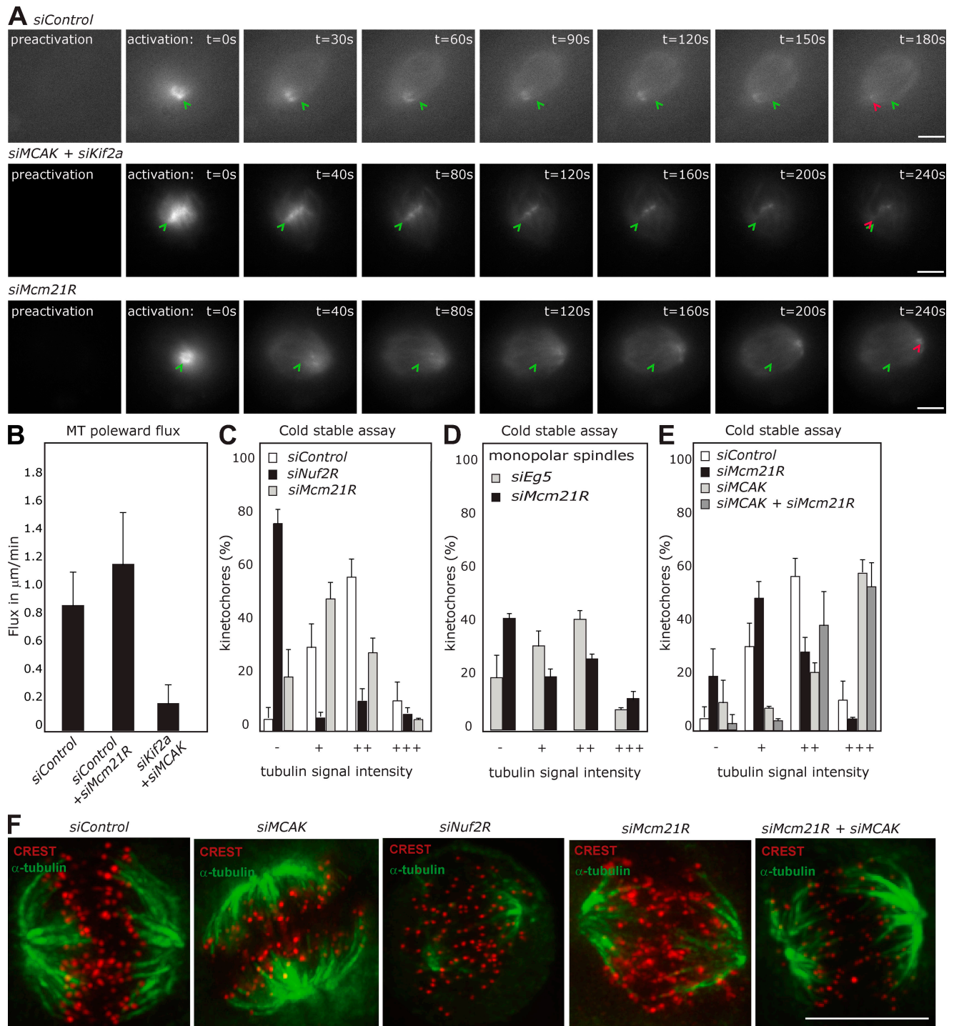
Figure 2. Depletion of Mcm21R reduces the number of stable k-fibers. (A) Successive frames every 30 or 40 s after photoactivation of stable PA-GFP- \alpha -tubulin/hTERT-RPE1 cells treated either with siControl , siMcm21R , or siMCAK + siKif2A RNAs. Green arrowheads mark the initial position of a photoactivated mark, and red arrowheads show the final position of the mark. (B) Quantification of poleward MT flux rate in cells treated with siControl ( n = 9 ), siMcm21R ( n = 9 ), or siMCAK + siKif2A ( n = 5 ) RNAs. (C–E) Quantification of stable k-fibers in cold-treated cells (for methodology, see Fig. S2, available at http://www.jcb.org/cgi/content/full/jcb.200809055/DC1 ). Bar graphs indicate the percentage of kinetochores lacking attached MTs (–), having a weak attachment (+), a medium attachment (++), or a strong attachment (+++) in siControl ( n = 354 ), siNuf2R ( n = 204 ), and siMcm21R ( n = 273 )-treated cells with bipolar spindles (C), in siMcm21R ( n = 215 )- and siEg5 ( n = 212 )-treated cells with monopolar spindles (D), and in siControl ( n = 354 ), siMcm21R ( n = 273 ), siMCAK ( n = 238 ), and siMcm21R + siMCAK ( n = 219 )-treated cells with bipolar spindles (E). (F) Representative images from C and E of cold-treated cells stained with \alpha -tubulin antibodies (MTs; green) and CREST antisera (kinetochores; red). Error bars represent SEM. Bars, 10 \mu\text{m} .
