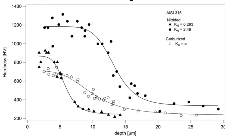
Fig.16: Hardness-depth profiles of AISI 316 nitrided at 445 °C (718 K) for 22 h in NH 3 -H 2 -N 2 gas mixtures, with nitriding potentials indicated, or carburized at 507 °C (780 K) for 6 h in a CO-H 2 -N 2 gas mixture. The lines are fitted by a Hill equation and show a sharper case-core transition for nitrided than for carburized material [42].
