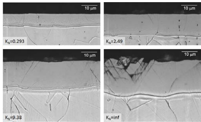
Fig.15: Cross sections of AISI 316 nitrided at 445 °C (718 K) for 22 h in NH 3 -H 2 -N 2 gas mixtures, at various nitriding potentials, K_N [41,46] .
