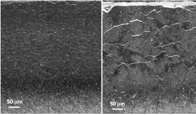
Fig.11: Cross sections of the diffusion zone in 33CrMoV12.9 nitrided at 520°C (793 K) for 100 h. The steels in have grain an average grain size of 15 μm (left) and 85 μm (reight). Network of (converted) carbides along grain boundaries develop [36].
