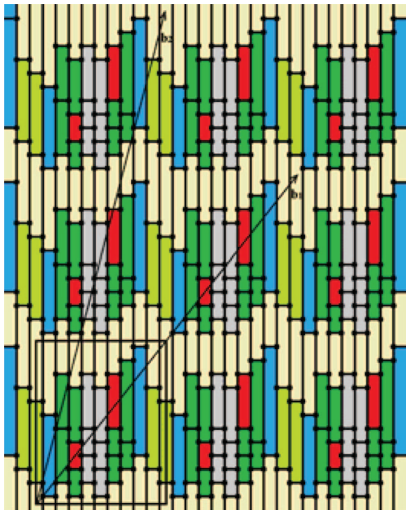
Figure 1. (Color online) Graph (n_6, n_7, n_5, (b_1, b_2)) = (1, 1, 2, 2, ((2, 2), (1, 3))) : tiling of the plane by heptagons, pentagons and hexagons where one row of hexagons is added at the top of the original LR cell and columns of heptagons and pentagons are separated by two stripes of hexagons, each. Super-cell vectors b_1 and b_2 are represented by the arrows and the unit cell by the rectangle.
