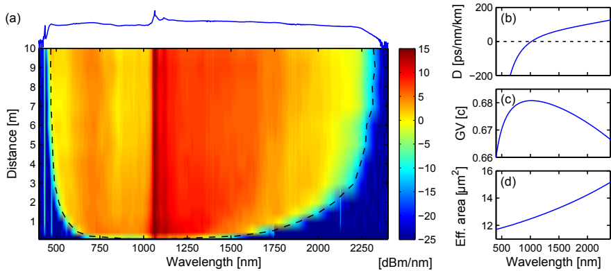
Figure 2.5: (a) Experimental cutback measurement of SC generation in a uniform PCF with hole-to-pitch ratio d/\Lambda = 0.85 and pitch \Lambda = 4.4 \mu\text{m} . (b)–(d) Calculated dispersion, GV and effective area, respectively. The fibre was pumped at 1064 nm with 10 ps pulses at 15 W average power and 80 MHz repetition rate. The dotted lines in (a) show the measured long-wavelength edge and the theoretically calculated GV matched blue edge.
