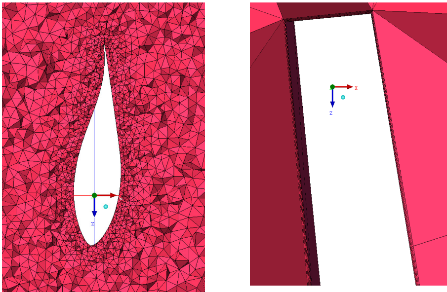
Figure 4: Cut through mesh at r=1.25 m, close up of blade and prism cells at trailing edge
