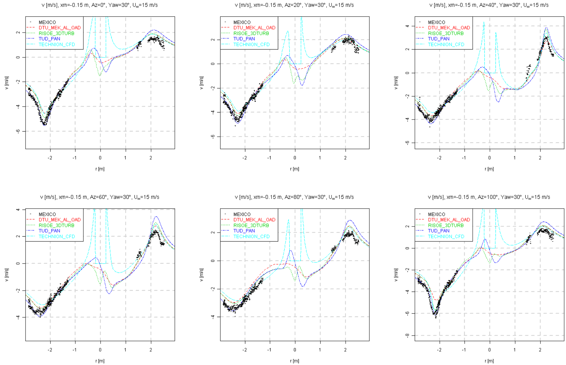
Figure 8.61 Radial traverse (upwind) of velocity in y-direction, Yaw=30°, U_\infty=15 m/s
