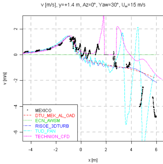
Figure 8.55 Axial traverse of velocity in y-direction, Yaw=30°, U ∞ =15 m/s
