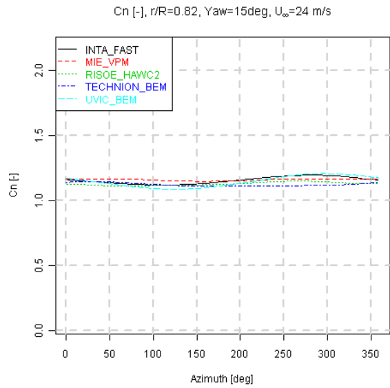
Figure 8.50 Normal force coefficient variation with azimuth angle, U ∞ =24 m/s, Yaw=15°
