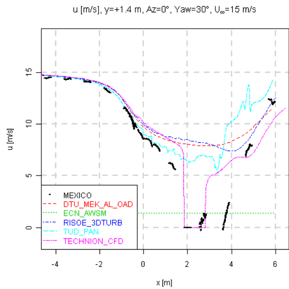
Figure 8.54 Axial traverse of velocity in x-direction, Yaw=30°, U ∞ =15 m/s
