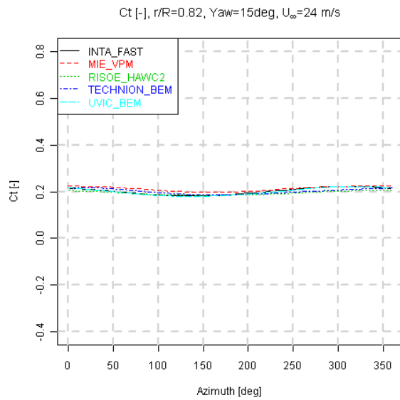
Figure 8.51 Tangential force coefficient variation with azimuth angle, U_{\infty}=24 \text{ m/s} , \text{Yaw}=15^{\circ}
