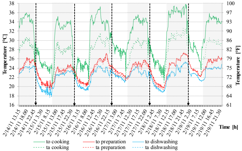
Fig. 3. Air & operative temperature ( t_a & t_o ) variations in different kitchen zone in winter
