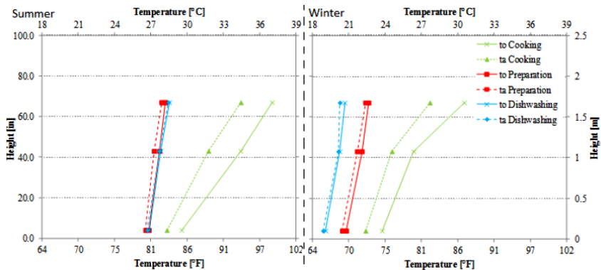
Fig. 2. Vertical Profile of Average Temperatures Distribution for Casual Kitchen
