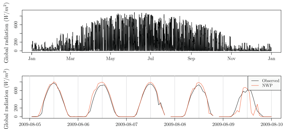
Fig. 3. The upper plot shows the time series of observed global radiation at DTU Byg covering the entire year 2009. In the lower plot the observations and NWP of global radiation at DTU Byg are shown for five days in August 2009.
