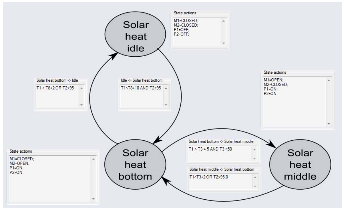
Figure 31. Control strategy.
