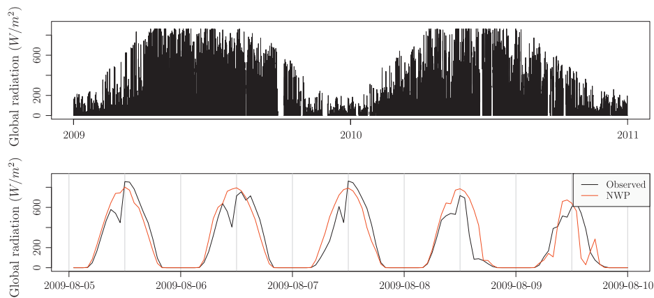
Fig. 2. The upper plot shows the time series of observed global radiation in Sønderborg. In the lower plot the observations and NWP of global radiation in Sønderborg are shown for 5 days in August 2009.
