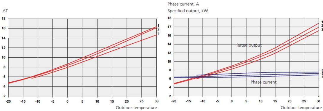
Figure 25. Temperature increase of water and power output as a function of the outdoor temperature for the het pump.
