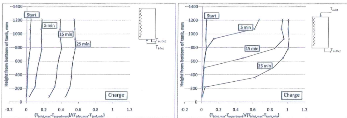
Fig. 2: Temperature profiles during charging tests without stratification inlet manifold. On the left with inlet from the bottom of the tank and on the right with inlet from the top of the tank.
