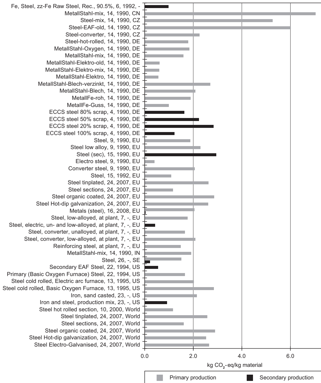
Figure 7: Emission of CO 2 -eq from the primary and secondary production of steel (Paper VI). Numbers in names refer to sources in Table 9. “-”: No data found.
