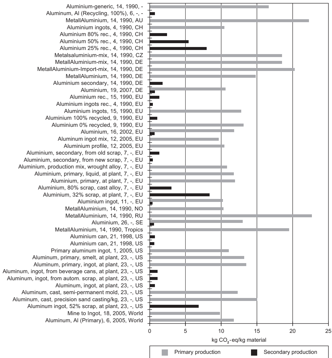
Figure 8: Emission of CO 2 -eq from the primary and secondary production of aluminium (Paper VI). Numbers in names refer to sources in Table 9. “-”: No data found.
