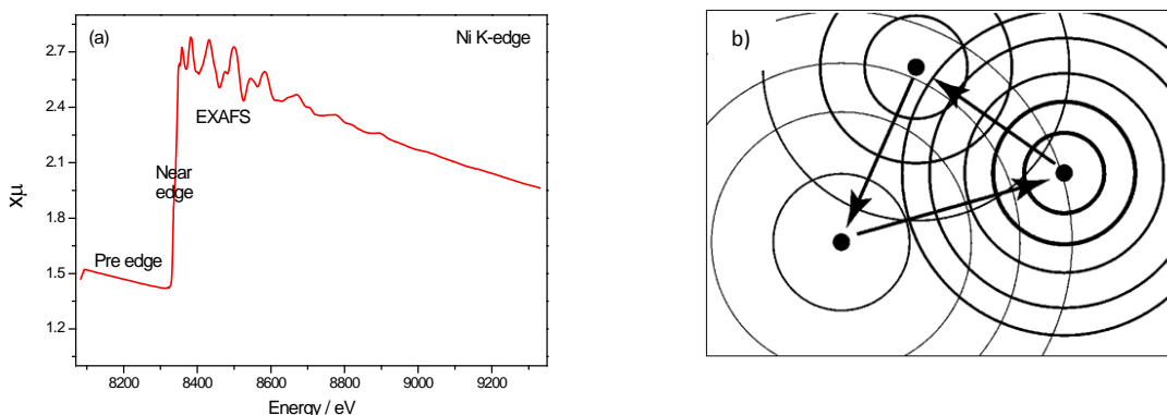
Figure 3.2. (a) A XAS spectrum of an as-prepared Ni 5 Ga 3 /SiO 2 catalyst and (b) simplified illustration of a multiple scattering event (33).
