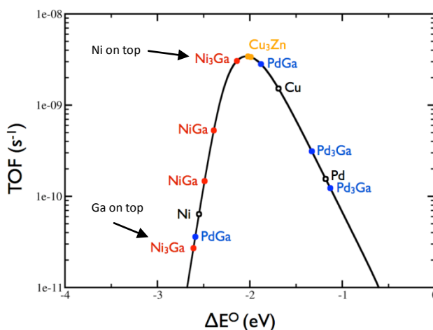
Figure 1.1. Turnover frequency values for \text{CO}_2 hydrogenation to methanol calculated as a function of oxygen binding energy. Reaction conditions are 500 K, 1 bar, \text{CO}_2 : \text{H}_2 ratio 1:3 (27)
