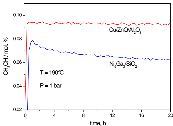
Figure 6.16. Deactivation behavior of Ni 5 Ga 3 /SiO 2 and Cu/ZnO/Al 2 O 3 catalysts.
