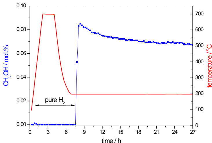
Figure 6.15. Catalytic activity of the Ni 5 Ga 3 catalyst supported on SiO 2 nanospheres.
