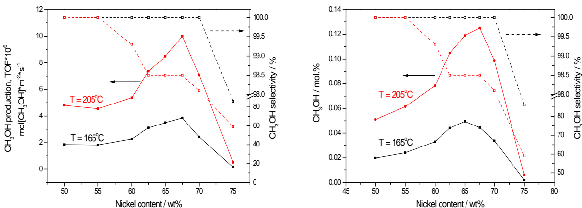
Figure 5.13. Activity of the Ni a Ga b /SiO 2 catalysts normalized to (a) surface area of active metals and (b) molar amount of active metals.
