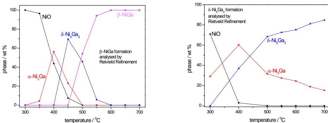
Figure 5.7. Rietveld refinement analysis of the phases formed during temperature programmed reduction of metal nitrates to form (a) NiGa/SiO 2 and (b) Ni 5 Ga 3 /SiO 2 .
