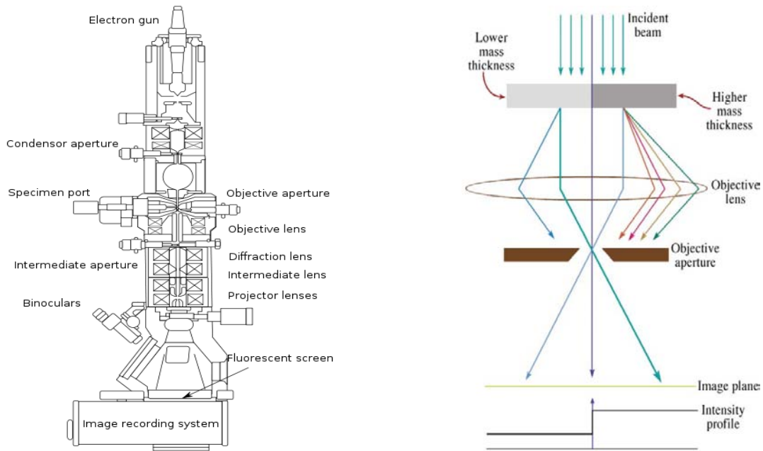
Figure 3.3. (a) Schematic drawing of a TEM apparatus and (b) image formation scheme due to mass thickness difference (35).
