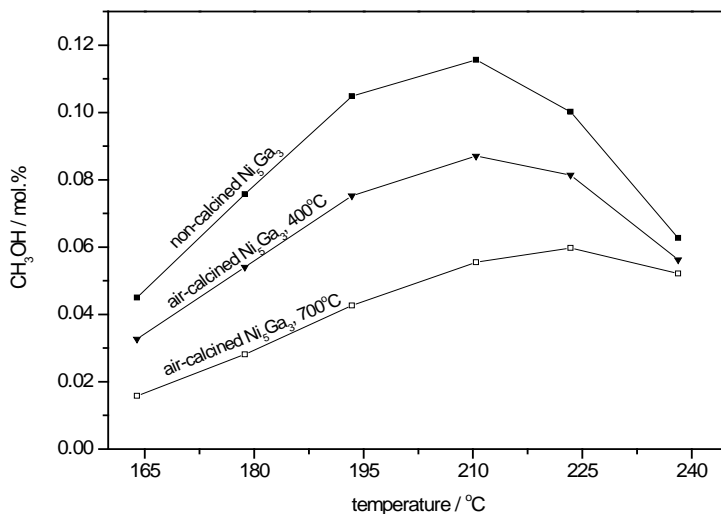
Figure 5.15. Activity dependence of a Ni 5 Ga 3 /SiO 2 catalyst on calcination temperature. P = 1 bar, CO 2 (75%)/ H 2 (25%) mixture.
