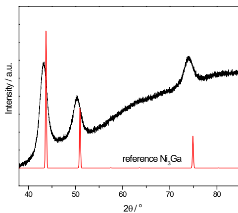
Figure 6.2. Ex-situ XRD test of the Ni 5 Ga 3 /SiO 2 catalyst after the accelerated ageing test.
