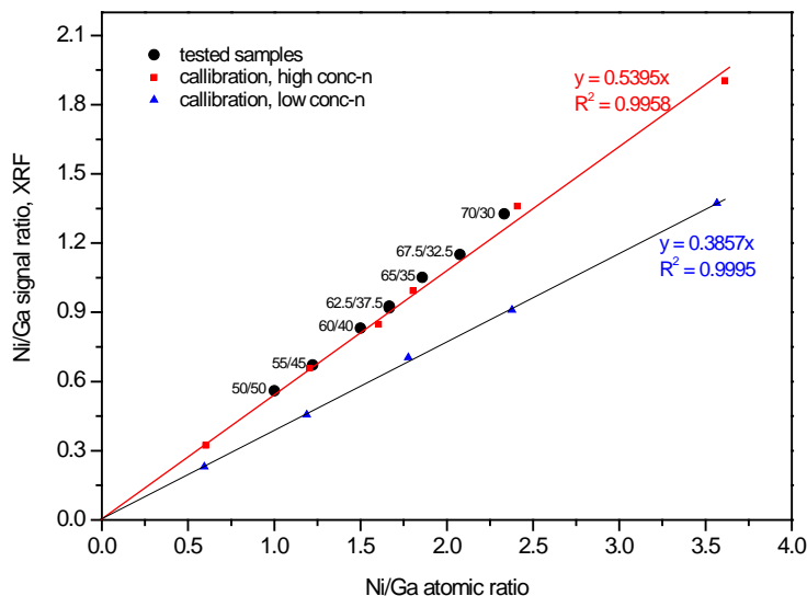
Figure 5.14. Quantification of the Ni/Ga ratio in the Ni_aGa_b/SiO_2 catalysts using X-Ray Fluorescence.
