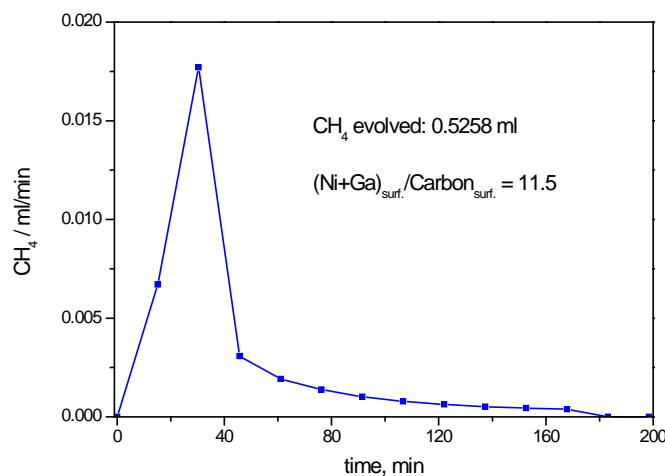
Figure 6.13. Methane evolution upon regeneration of the Ni 5 Ga 3 /SiO 2 catalyst. T = 300°C, pure H 2 flow.
