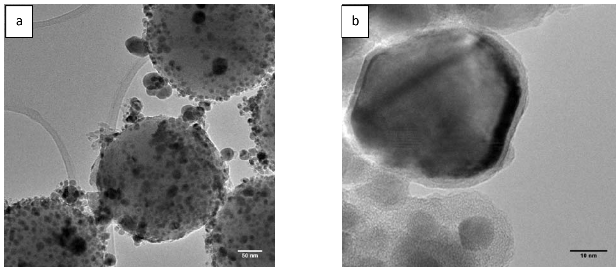
Figure 6.15. (a) TEM and (b) HRTEM images of the Ni 5 Ga 3 catalyst supported on SiO 2 nanospheres.
