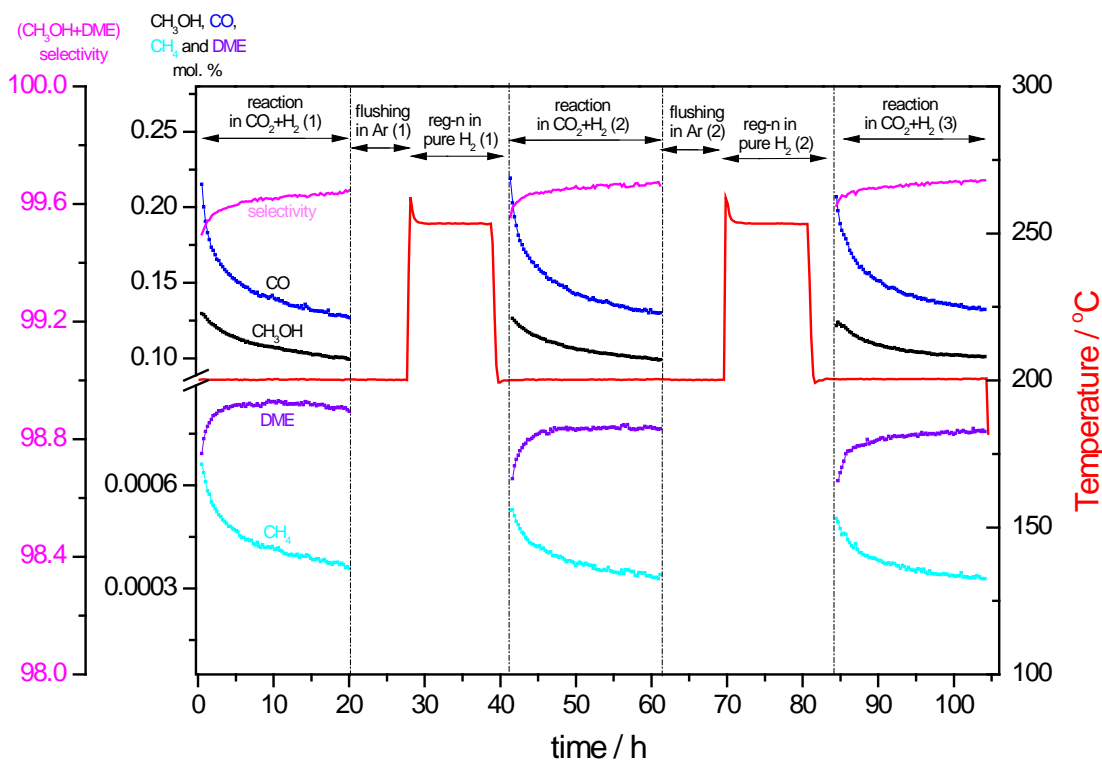
Figure 6.10. Methanol synthesis experiment followed by flushing and further regeneration of the catalyst. Reaction conditions: 25% CO 2 in H 2 , atmospheric pressure.
