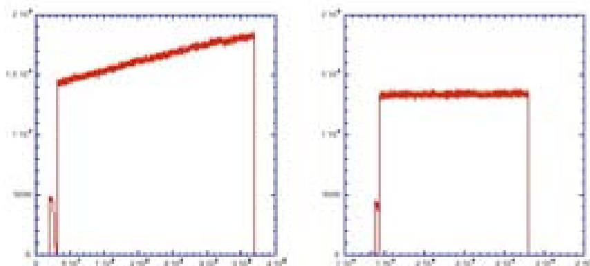
FIGURE 1. Leaky target (right) vs. tight target (left), reflected in the neutron counting rate.
