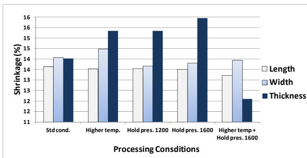
Figure 9: Shrinkage of sintered parts in length, width and thickness.
