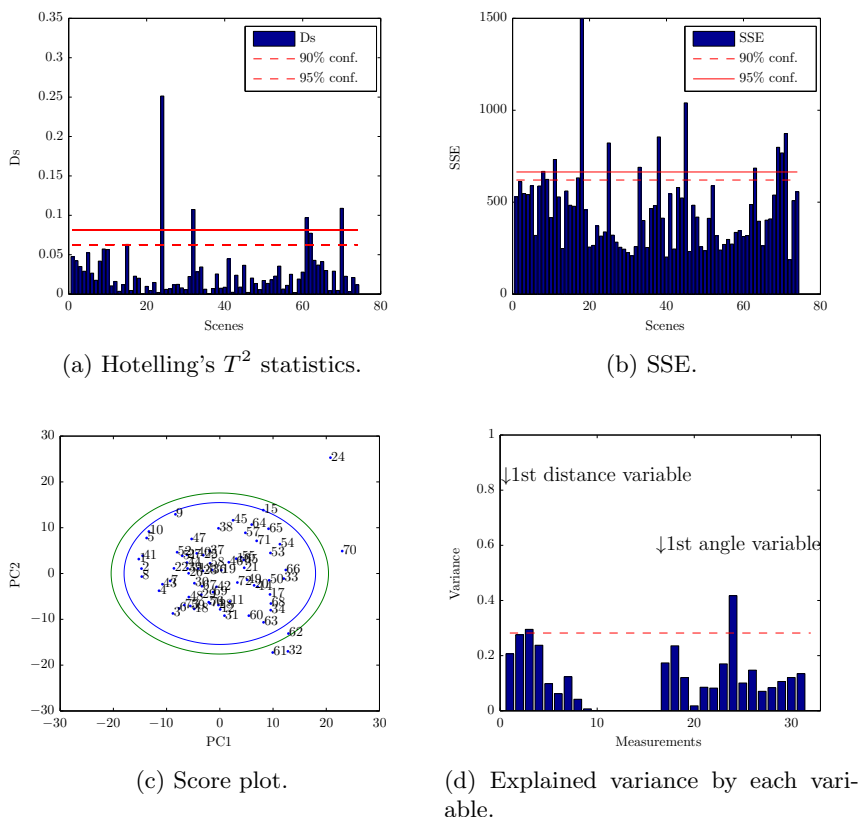
Fig. 3: Training data.
