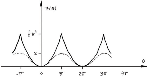
Fig. 2: Periodic parametric potential (18) originating from the potential in (2). The dashed curve corresponds to the Wilson analogue [14] of the Manton action and is not considered in the present work.
