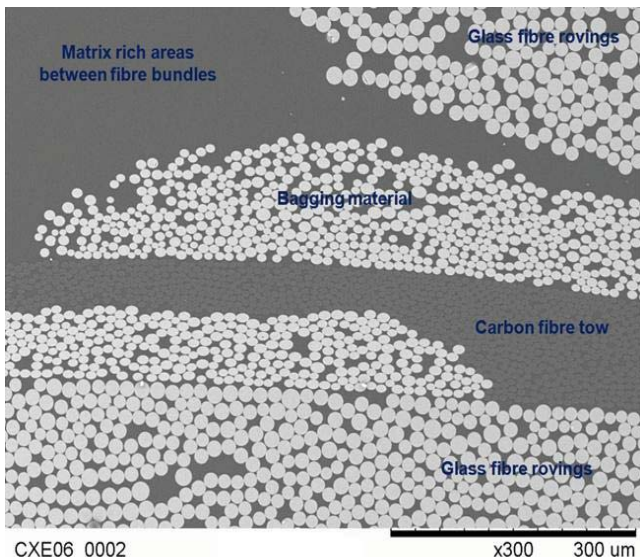
Figure 2. Microscopic image for a hybrid fabric carbon/glass/epoxy composite
