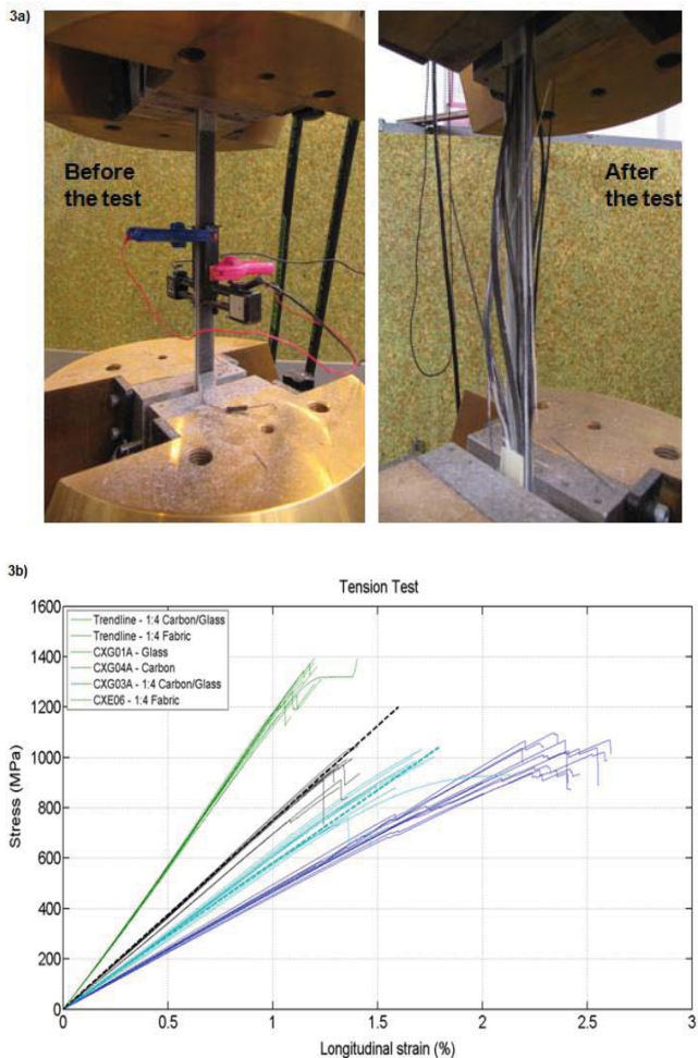
Figure 3. a. Tensile test setup with mechanical extensometers and specimen, before and after test b. Comparison of stress-strain graphs – hybrid and non-hybrid carbon/glass composites
