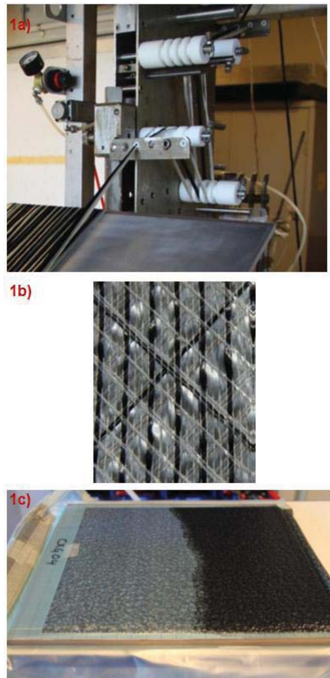
Figure 1. a. Filament winding setup b. Carbon/glass hybrid fabric c. Vacuum infusion process trails
