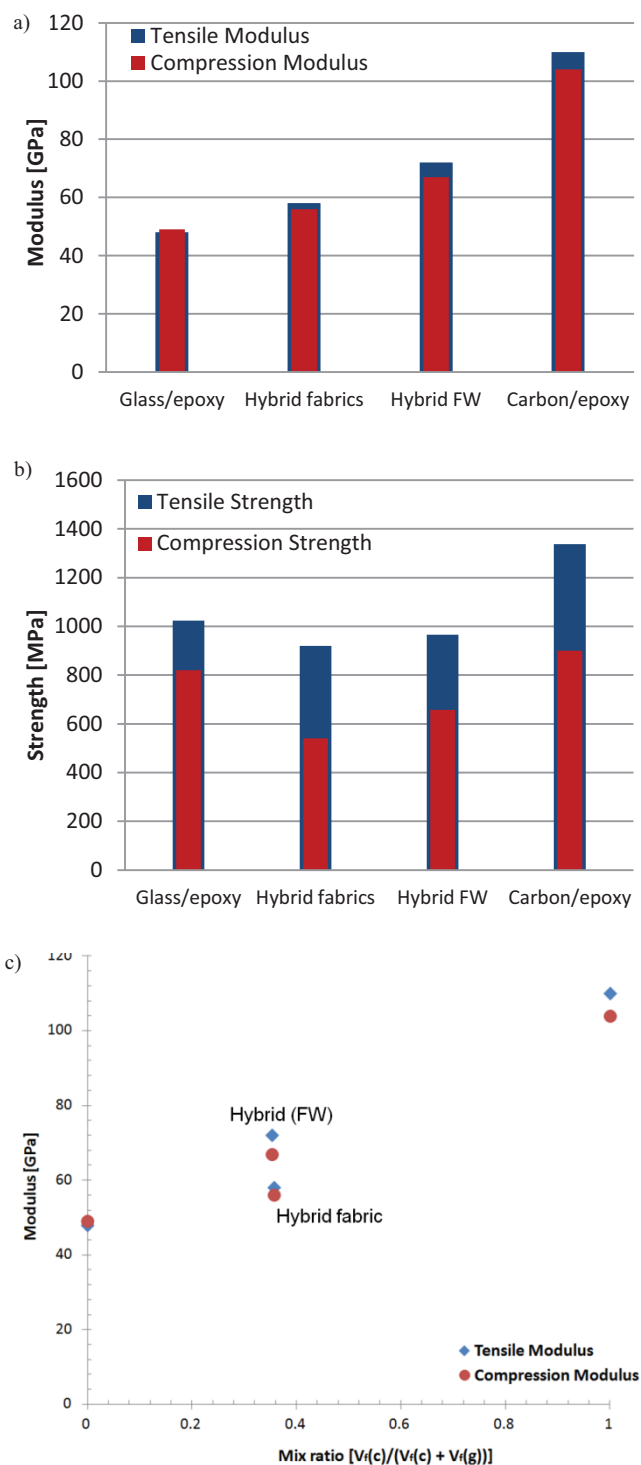
Figure 5.a. Bar graph demonstrating the comparisons of hybrid and non-hybrid stiffness
