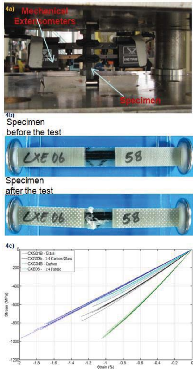
Figure 4.a. Test specimen fixed in the MCL fixture. b. Specimens before and after the compression test c. Comparison of stress-strain graphs – hybrid and non-hybrid carbon/glass composites
