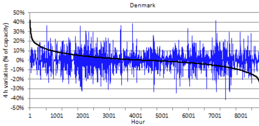
Figure 43. Time series and duration curve of 4 h production variation in Denmark 2010.
