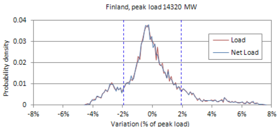
Figure 78. Variability of load and net load in Finland, year 2010.
