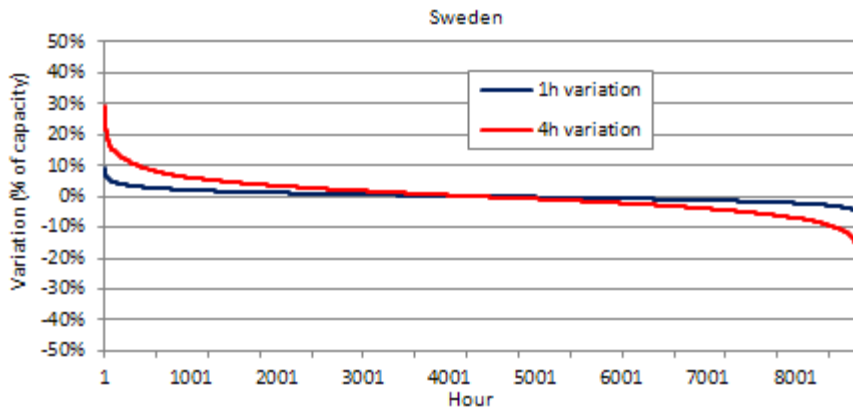
Figure 42. Duration curves of 1 hour and 4 hour variation in Sweden 2010.
