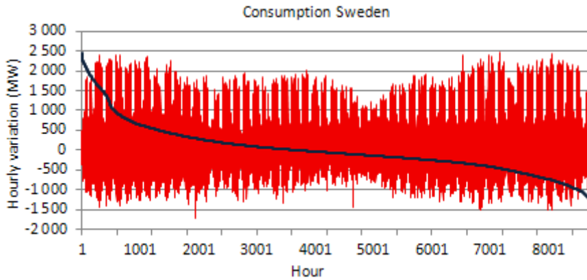
Figure 66. Hourly variations of consumption in Sweden 2010.
