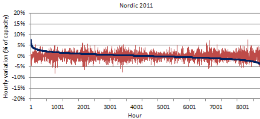
Figure B8. Hourly variation of wind power production in Nordic countries 2011.
