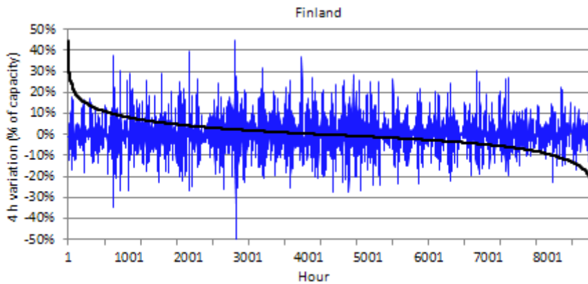
Figure 44. Time series and duration curve of 4 h production variation in Finland 2010.
