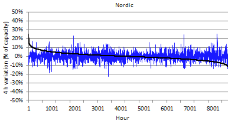
Figure B15. 4 hour variation in Nordic countries 2009.
