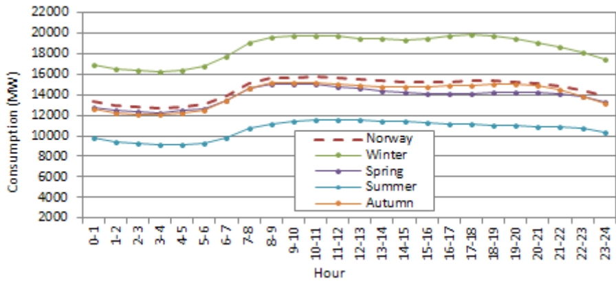
Figure 59. Diurnal pattern of consumption Norway 2009–2011.
