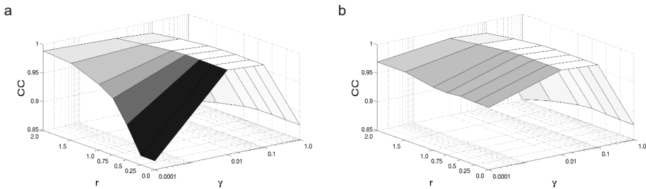
Figure 10. Plots depicting the CC over the range of studied r and \gamma parameters of images reconstructed from noisy data from 128 views (a) and 9 views (b). For these images, the projection data were generated by the system matrix.
