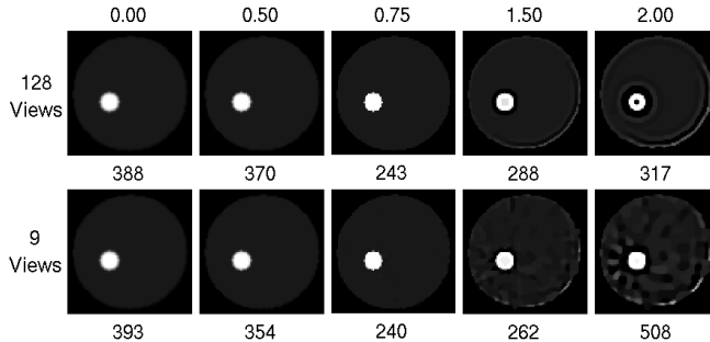
Figure 7. Intermediate images f and the number of meaningful sparsity coefficients reconstructed from 128 and 9 noiseless inverse crime data using \gamma = 0.0001 .
