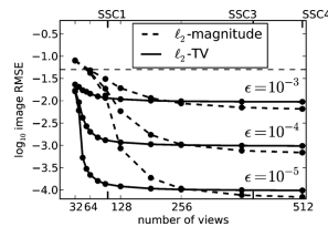
Fig. 10. Image RMSE, \delta , for \ell_2 -magnitude and \ell_2 -TV reconstructions, as in Fig. 6 for varying \epsilon , computing X with ray-tracing and nearest-neighbor interpolation. N_{\text{bins}} is fixed at 512. The labels SSC1, SSC3, and SSC4 are the sufficient-sampling conditions discussed in Section IV-A.
