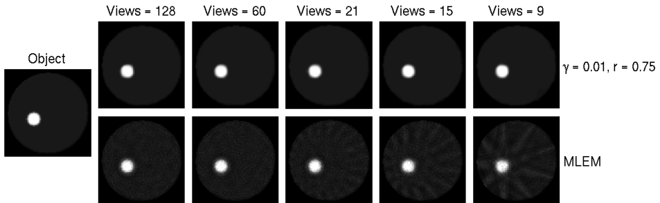
Figure 13. Images reconstructed from noisy projections using the proposed algorithm and MLEM for varying sampling cases. For these images, the projection data were generated by the system matrix.
