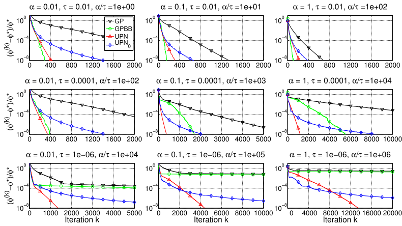
Fig. 3 Convergence histories (\phi(x^{(k)} - \phi^*)/\phi^* vs. k for TI with \alpha = 0.01, 0.1 and 1 and \tau = 10^{-2}, 10^{-4} and 10^{-6} . Methods are Gradient Projection ( GP ), Gradient Projection Barzilai-Borwein ( GPBB ), Unknown Parameter Nesterov ( UPN ), and UPN with \mu_k = 0 ( UPN_0 ). As the ratio \alpha/\tau increases, which implies an increased Q and a computationally more difficult problem, UPN and UPN_0 scale significantly better. For high accuracy solutions UPN is always competitive
