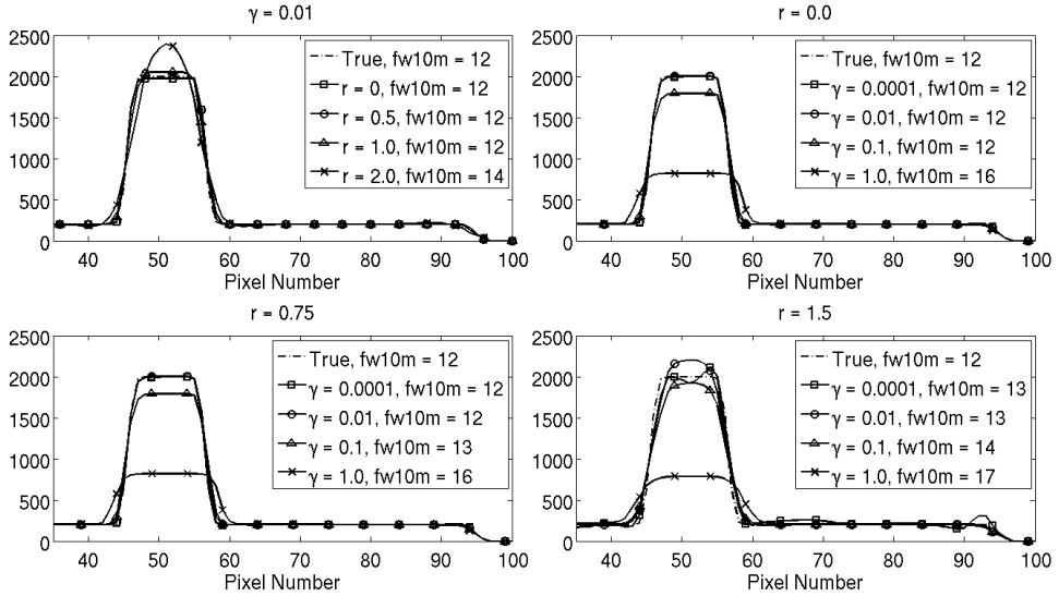
Figure 6. Central diagonal profiles through images reconstructed from noiseless inverse crime data from 9 views using the proposed algorithm with varying values of r and \gamma .
