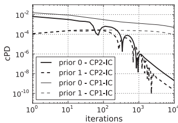
FIG. 9. The conditional primal-dual gap for IC shown for CP2-IC and CP1-IC. This gap is computed by taking the difference between the primal and dual objectives in Eqs. (13) and (14), respectively, after removing the indicator in the primal objective: cPD = \frac{1}{2} \|f - f_{prior}\|_2^2 + \frac{1}{2} \|X^T y\|_2^2 + \epsilon' \|y\|_2 + g^T y - f_{prior}^T (X^T y) / \text{size}(f) . The absolute value is used because the argument can be negative, and we normalize by the number of pixels \text{size}(f) so that the primal objective takes the form of a mean square error. The prior image f_{prior} for this computation is explained in the text. The comparison between CP2-IC and CP1-IC shows quantitatively the impact of the acceleration afforded by CP Algorithm 2.
