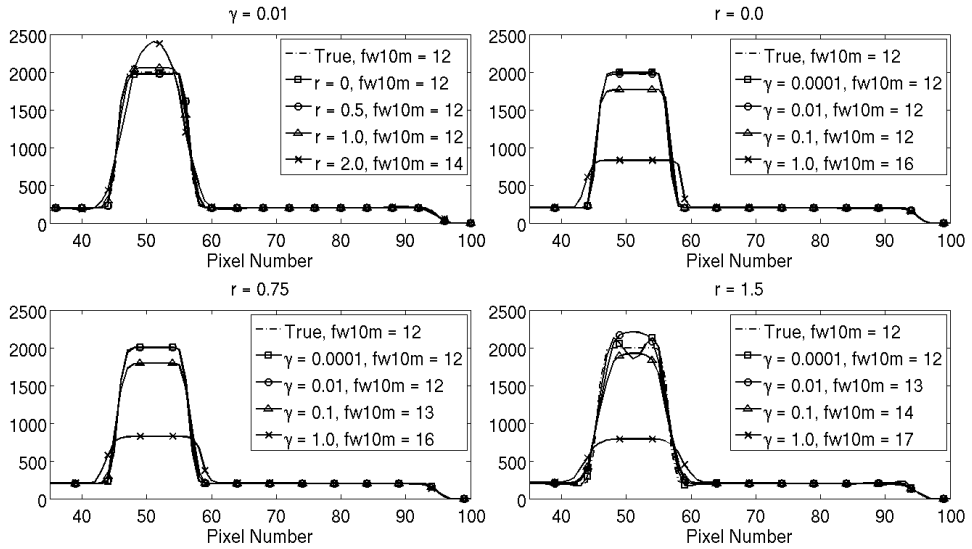
Figure 3. Central diagonal profiles through images reconstructed from noiseless inverse crime data from 128 views using the proposed algorithm with varying values of r and \gamma .
