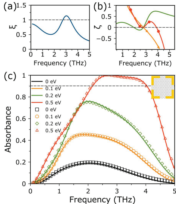
Fig. 6. (a) Real part of normalized surface conductivity of two graphene fishnet layers \zeta = 1 at 2.7 THz. (b) Imaginary part \zeta (green line) defines the value of dielectric thickness h , so that quickly changing \gamma \cot \Phi (red line with circles) compensate \zeta and give \zeta + \gamma \cot \Phi = 0 (orange line with triangles) at the same frequency 2.7 THz. (c) Absorbance of the device is tuned by Fermi energy [0 (black), 0.1 (orange), 0.2 (green), 0.5 (red) eV]. The analytical predictions (lines) are in a perfect correspondence with full-wave simulation results (symbols). The working bandwidth at A \geq 0.9 is 1.9 THz.
