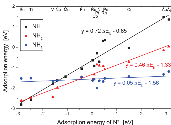
FIG. 3. The scaling relations for NH_x species on the relaxed M12 nanoclusters consisting of transition metals. The adsorption geometries are chosen as the most stable calculated ones.
