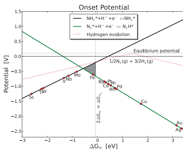
FIG. 6. Volcano plot for the associative and dissociative mechanism with the free energy \Delta G_{N^*} as a descriptor. The competing reaction of creating hydrogen on the surface is also shown as the dotted lines. The two solid lines indicate the limiting potential for the associative mechanism. For the dissociative mechanism the gray area is added as a potential area for where it could be more favorable to go through the dissociative mechanism. The efficiency in this area is dependant on the dissociation of the N_2 molecule on the surface. At the top of the gray area the dissociative mechanism will be comparable to HER.
