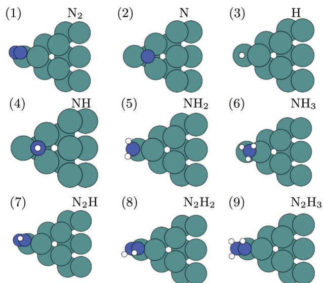
FIG. 2. The most stable adsorption sites for the reaction intermediates in both the dissociative and associative mechanism on the ruthenium M12 nanocluster. The dark atoms are nitrogen, the small atoms are hydrogen and the light atoms are ruthenium. The adsorption sites for the adsorbates presented for the M12 nanocluster are only representative for the type of adsorption site (hollow, bridge, on-top) and not the actual bonding site for the other metals, which means a N atom could bind more strongly to another hollow site on a different metal studied in this work.
