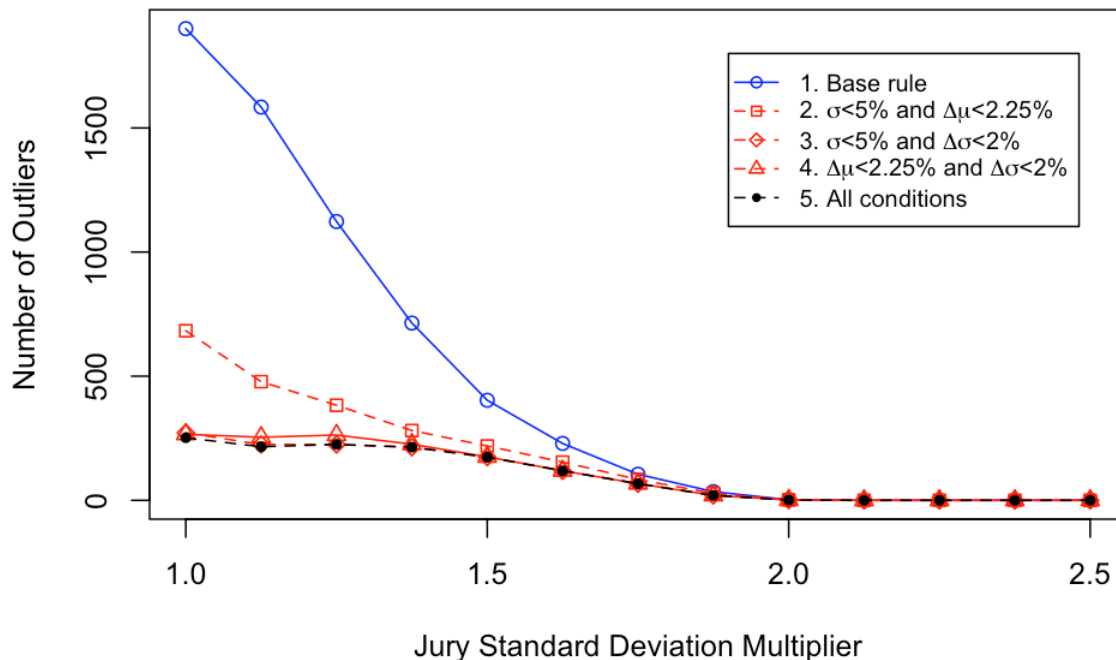
Figure 2. Number of Flagged Outliers as a Function of the Standard Deviation Multiplier Value with Two Conditions Active at a Time
