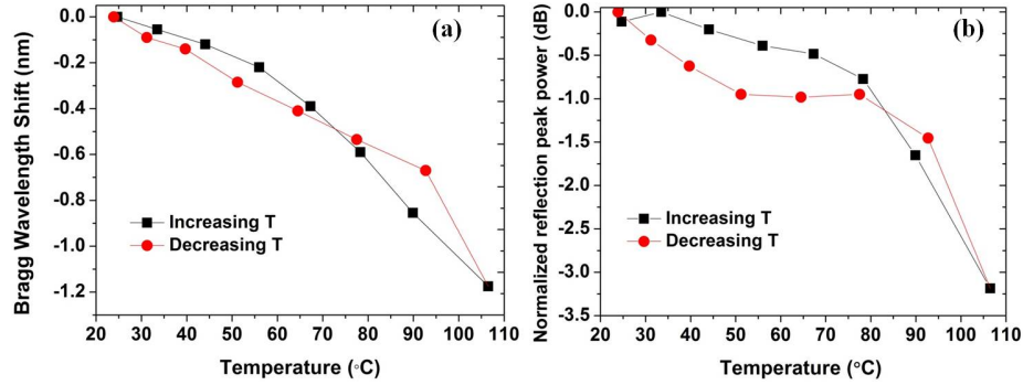
Fig. 2. Temperature response of the FBG in the 130 μm fiber shown in Fig. 1. (a) Bragg wavelength shift versus temperature. (b) Normalized reflected peak power versus temperature.
