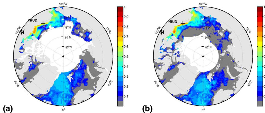
Fig. 5. Spatial distribution of temporal correlation coefficient between tide gauge and altimetric data at Prudhoe Bay: (a) DUACS data set, (b) MyOcean V2p data set. The same color scale is used for all plates.
