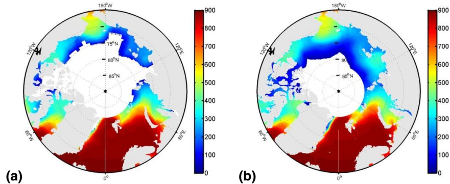
Fig. 1. The number (in weeks) of the valid data in the Arctic Ocean from (a) DUACS data set and (b) MyOcean V2p data set.
