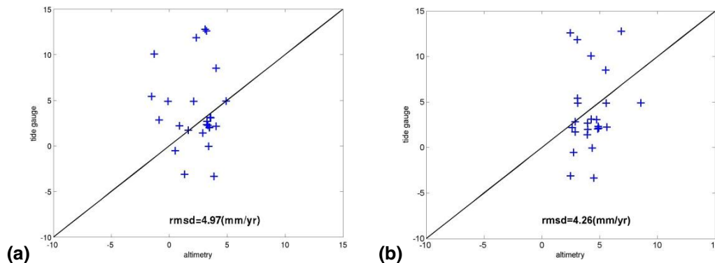
Fig. 9. Comparison between collocated sea level trend ( \text{mm yr}^{-1} ) from tide gauge and altimetric: (a) DUACS data set, (b) MyOcean V2p data set.
