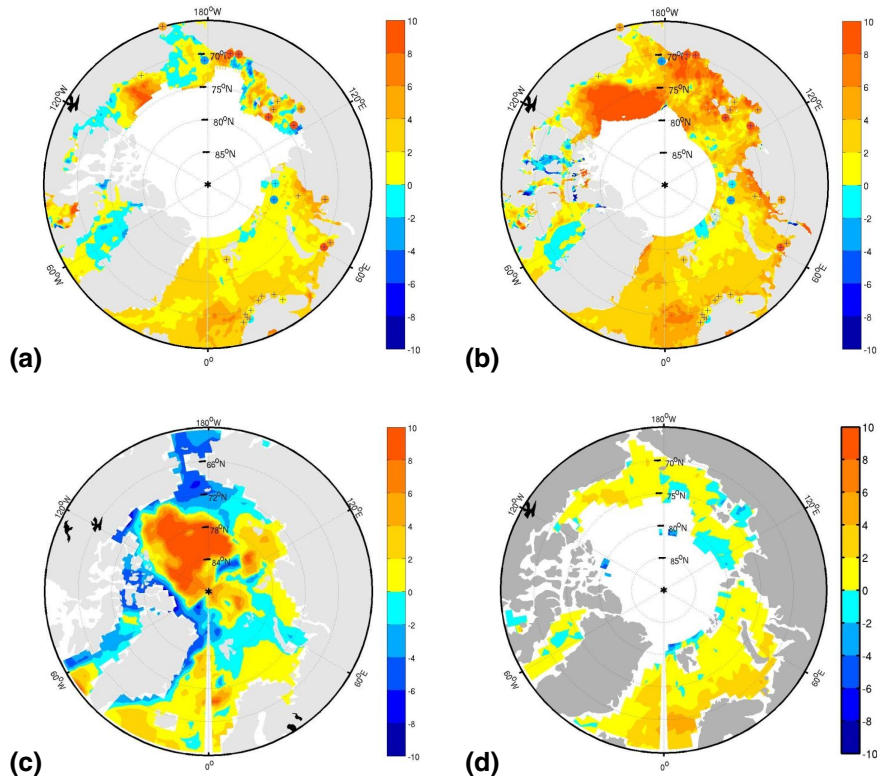
Fig. 8. Spatial distribution of sea level trend ( \text{mm yr}^{-1} ) from: (a) DUACS data set (1993–2009), (b) MyOcean V2p data set (1993–2009), (c) SODA (1993–2008) and (d) RADS (1993–2009). The same color scale is used for all plates. The amplitude of annual signal from tide gauge data (1993–2009) is illustrated in panels (a) and (b) with the same color scale. The pluses in panels (a) and (b) denote the positions of the selected tide gauges.
