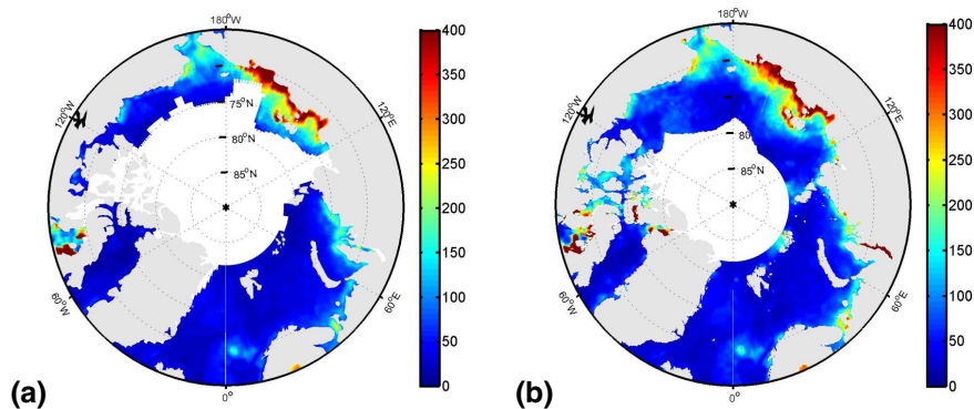
Fig. 3. SLA variance ( \text{cm}^2 ) in the Arctic Ocean from (a) DUACS data set and (b) MyOcean V2p data set. The same color scale is used for all plates.
