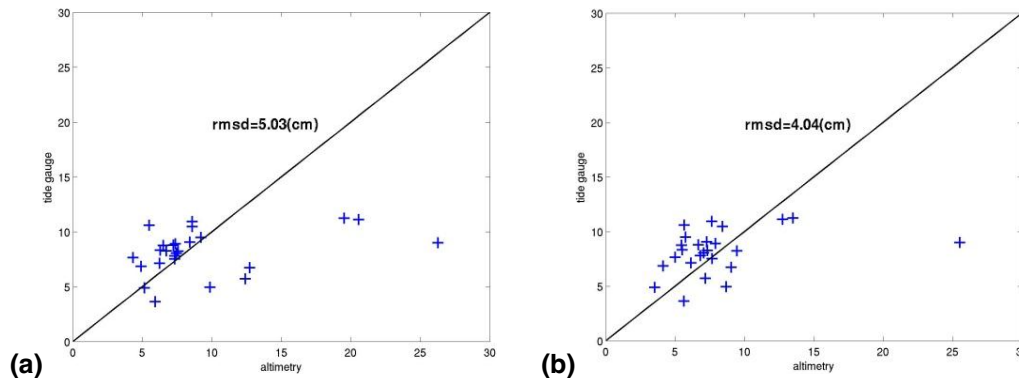
Fig. 7. Comparison between collocated amplitude of annual signal (cm) from altimetry and tide gauge data: (a) DUACS data set, (b) MyOcean V2p data set.
