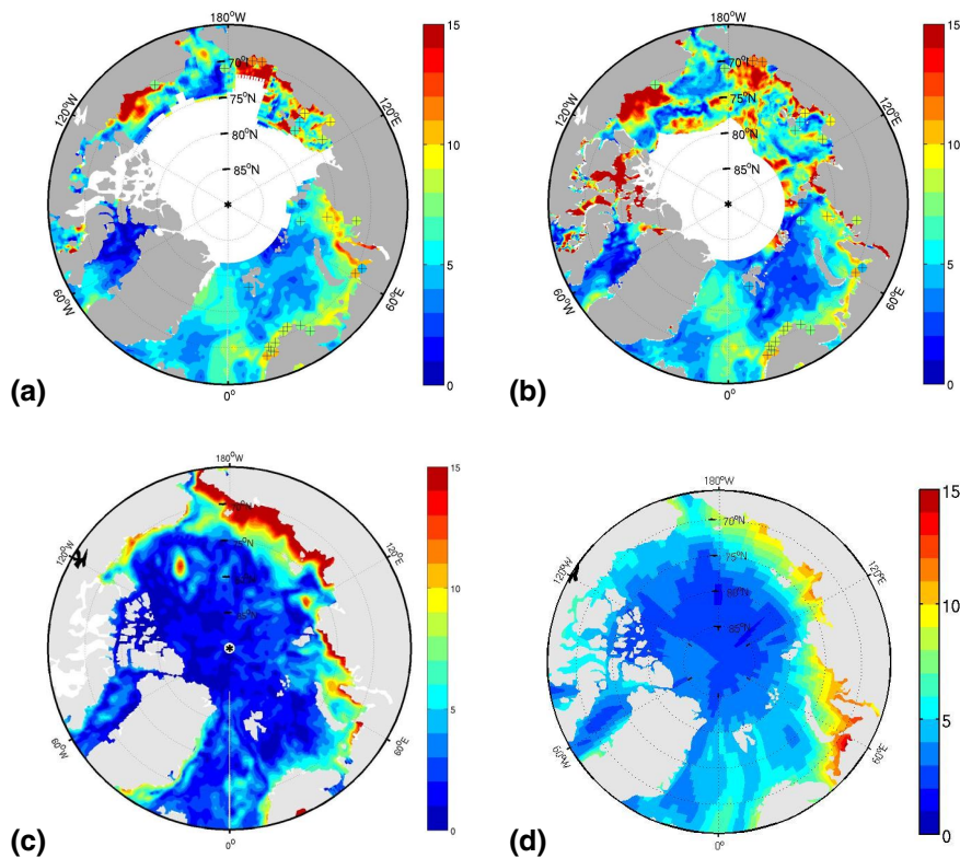
Fig. 6. Spatial distribution of amplitude of annual signal (cm) estimated from: (a) DUACS data set, (b) MyOcean V2p data set, (c) SODA and (d) DTU10ANN. The same color scale is used for all plates. The pluses in panels (a) and (b) denote the positions of the selected tide gauges.
