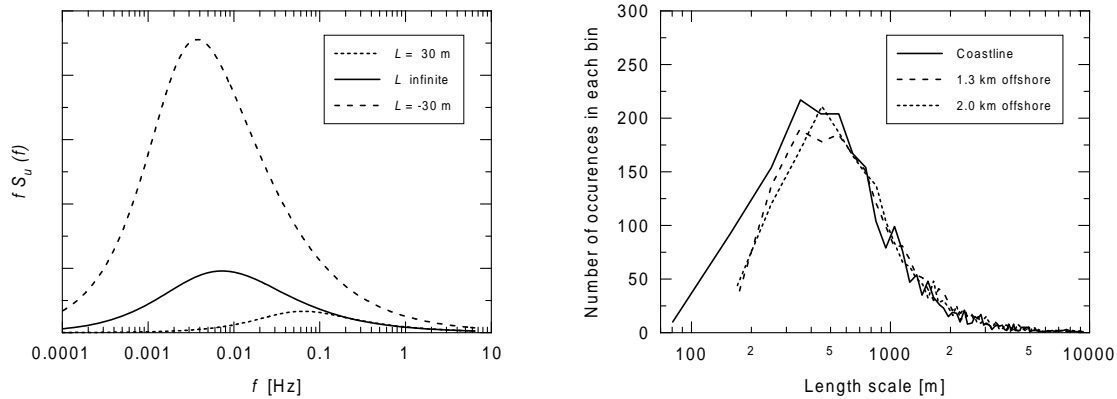
Figure 8. (a) Model spectra of the streamwise velocity component 50 m a.g.l. in flat terrain for neutral ( L infinite), stable ( L = 30 m) and unstable ( L = -30 m) conditions, where L is the Monin-Obukhov length [34, 35, 36]. The areas under the curves are proportional to the variances. (b) Probability distribution of length scales from the Vindeby site at heights of 48 m. Length scales were derived by the ‘half variance’ method.
