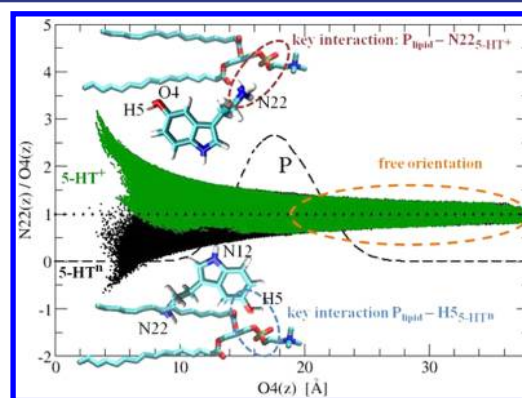
Figure 4. Scatter plot of the ratio of \text{N}_{22,5\text{-HT}}(z) and \text{O}_{4,5\text{-HT}}(z) position as a function of \text{O}_{4,5\text{-HT}}(z) position. The z -axis is along the bilayer normal, and the center of mass of the bilayer is located at z = 0 . Black, DPPC/ 5\text{-HT}^n ; green, DPPC/ 5\text{-HT}^+ . As a reference, the probability distribution, \text{P}_{\text{lipid}} is included (see Figure 2 for details). \text{P}_{\text{lipid}} is scaled by a factor of 20 ( y -axis) to show it on the same plot. The graph specifies the orientation of 5-HT and schematically shows the specific interactions observed between lipid and 5-HT. In the water phase, free orientation is observed, whereas depending on the protonation state of 5-HT, two distinct orientations of 5-HT are seen. Top: 5\text{-HT}^+ ; primary amino group points to the bilayer water interface. Key interaction: \text{P}_{\text{lipid}}-\text{N}_{22,5\text{-HT}^+} . Bottom: 5\text{-HT}^n ; primary amino group points into the bilayer region. Key interaction: \text{P}_{\text{lipid}}-\text{H}_{5,5\text{-HT}^n} .
