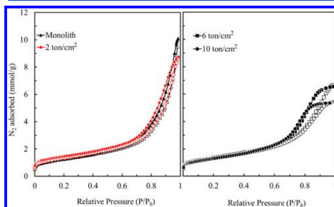
Figure 2. \text{N}_2 isotherms of \text{V}_2\text{O}_5\text{--}\text{WO}_3/\text{TiO}_2\text{--}\text{sepiolite} catalyst samples before and after pelletizing at various pressures.
