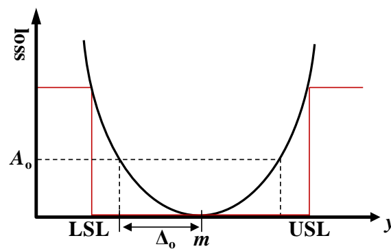
Figure 1. Quality loss function [Taguchi et al. 2005]
