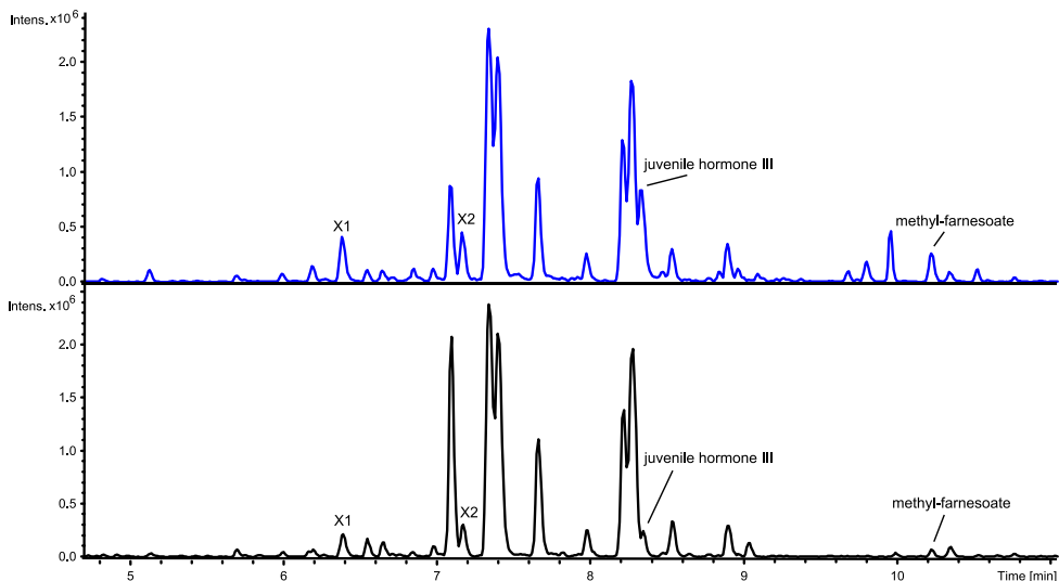
Figure 4.45 UHPLC-HRMS ESI+ BPC of the reference strain (bottom) and the strain where smrA (top) is expressed grown on CYA at 37°C for seven days.
