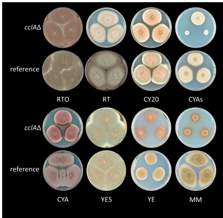
Figure 4 The appearance of the reference strain compared to the ccIAΔ strain cultivated for seven days at 37°C on RTO, RT, CY20, CYAs, CYA, YES, YE, and MM medium.
