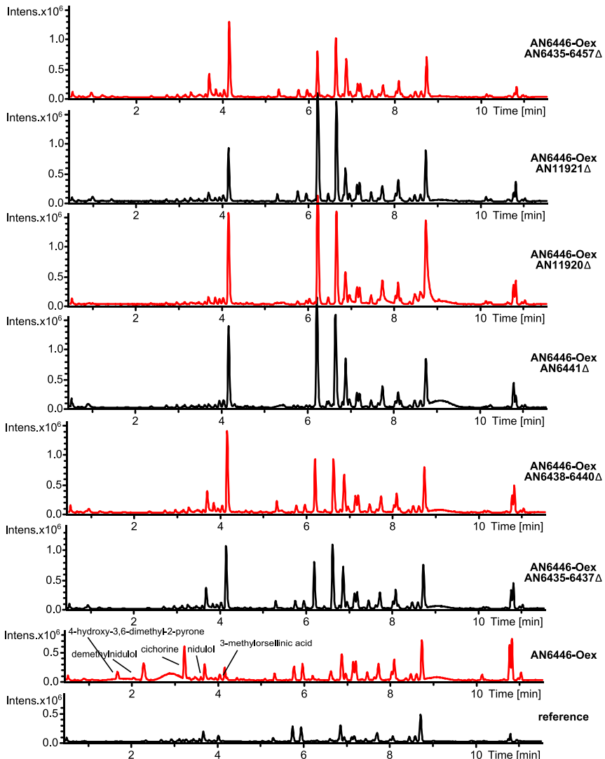
Figure 4.28 UHPLC-TOF-MS ESI+ BPC of the micro-extracts of the (from bottom to top) reference AN6446-Oex, AN6446-Oex AN6435-6437 \Delta , AN6446-Oex AN6438-6440 \Delta , AN6446-Oex AN6441 \Delta , AN6446-Oex AN11920 \Delta , AN6446-Oex AN11921 \Delta , AN6446-Oex AN6435-6457 \Delta strains cultivated on MM medium for seven days at 37°C. The metabolites identified in the AN6446-Oex strain are missing in all the deletions.
