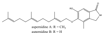
Figure 2.12 The structure of aspermidine A and B.
