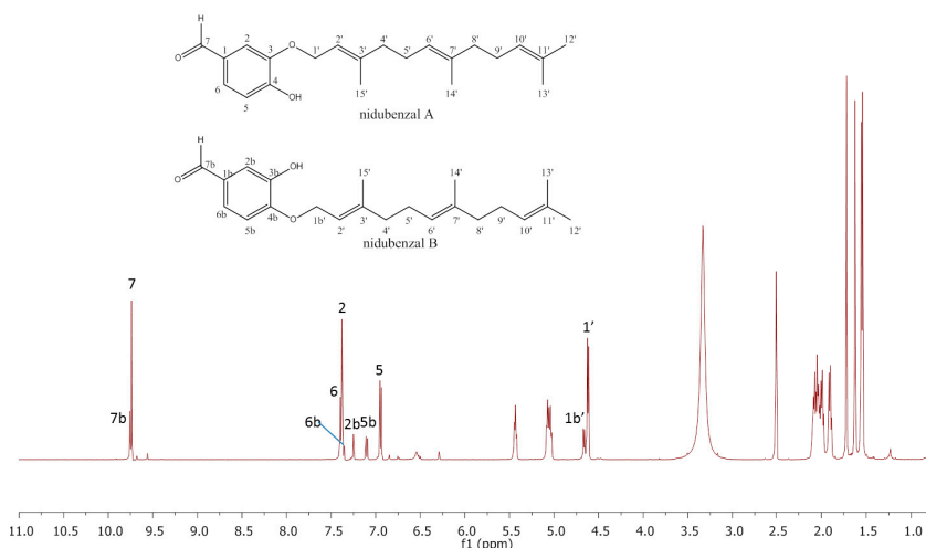
Figure 4.36 1 H-NMR spectrum of nidubenzal A and B in DMSO- d 6 . Which illustrates the two metabolites present in the solution.
