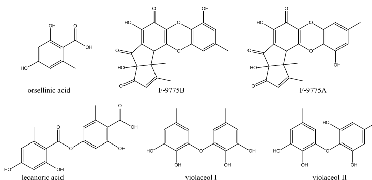
Figure 4.19 Structures of orsellinic acid, lecanoric acid, F-9775A, F-9775B, violaceol I, and violaceol II.
