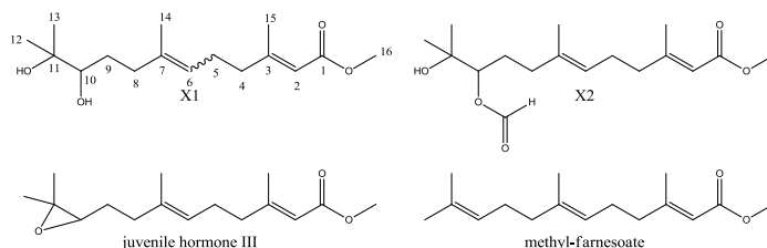
Figure 4.47 The structures of X1, X2, juvenile hormone III and methyl-farnesoate
