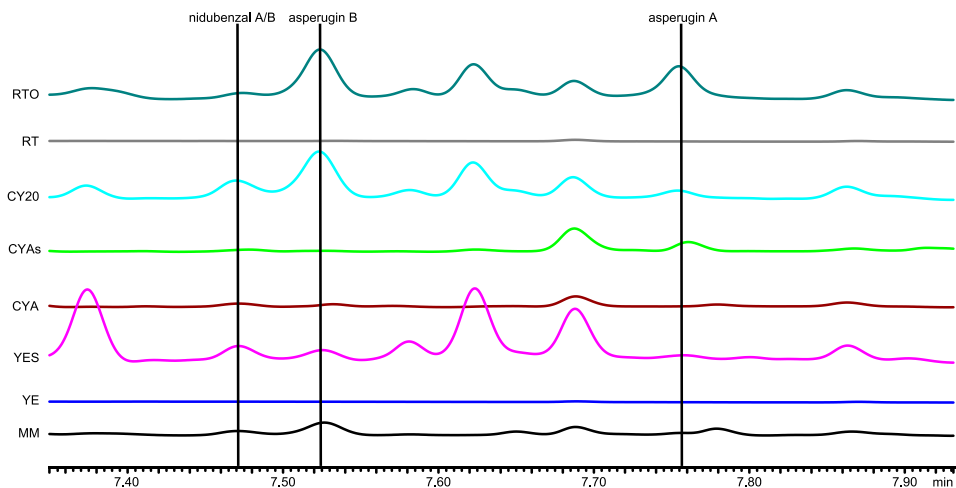
Figure 6 UHPLC-DAD chromatograms (210 nm) from seven to eight minutes of micro-extracts of the cclA \Delta on the eight different media. From top to bottom: RTO, RT, CY20, CYAs, CYA, YES, YE and MM.
