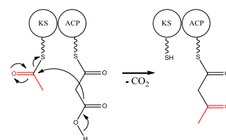
Figure 2.1 Chain extension of the PK chain in iPKSs through Claisen-like condensations of the extender and starter unit. The synthesis is started by binding a starter unit, here acetyl-CoA, to the KS domain and loading of the extender unit, here malonyl-CoA, to the ACP domain, releasing the CoA. The KS catalyzes the claisen-like condensation extending the polyketide chain by an acetate unit (marked in red) whereby \text{CO}_2 is released. To start another extension the polyketide chain is transferred back to the KS domain and the ACP domain is loaded with a new extender unit. Abbreviations: KS: \beta -ketosynthase, ACP: Acyl carrier protein.
