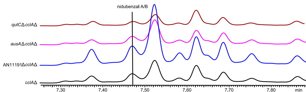
Figure 7 UHPLC chromatograms (210 nm) of micro-extracts of the qutCΔccl1Δ , ausAΔccl1Δ , AN11191Δ ccl1Δ and ccl1Δ strains after cultivation for seven days at 37°C on CY20 medium. The other parts of the chromatogram were also identical.
