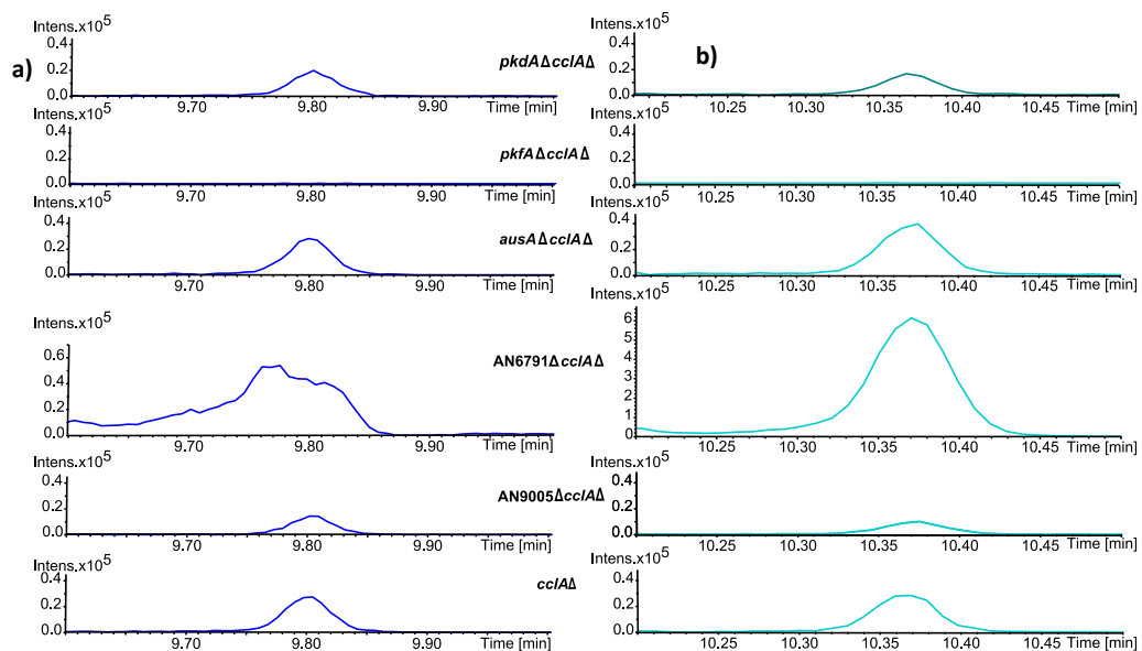
Figure 8 EIC of a) asperugin A (calc. [M-H]^- 401.23225±0.002) and b) asperugin B (calc. [M+H]^+ 387.21660±0.002) of micro-extracts of the (from top to bottom) pkdAΔccl1Δ , pkfAΔccl1Δ , ausAΔccl1Δ , AN6791Δ ccl1Δ , AN9005Δ ccl1Δ and ccl1Δ strains after cultivation on CY20 medium for seven days at 37°C.
