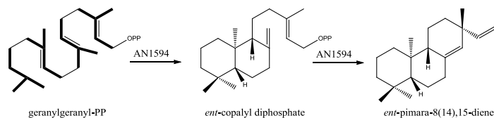
Figure 2.6 Folding and cyclization of the terpene ent -pimara-8(14),15-diene as proposed by Broman and co-workers (Broman 2012). The four isoprene units in geranylgeranyl-PP is highlighted in bold.
