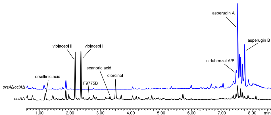
Figure 4.44 UHPLC chromatograms (210 nm) of micro-extracts of the orsAΔcclAΔ strain compared to the cclAΔ strain on CY20 medium.
