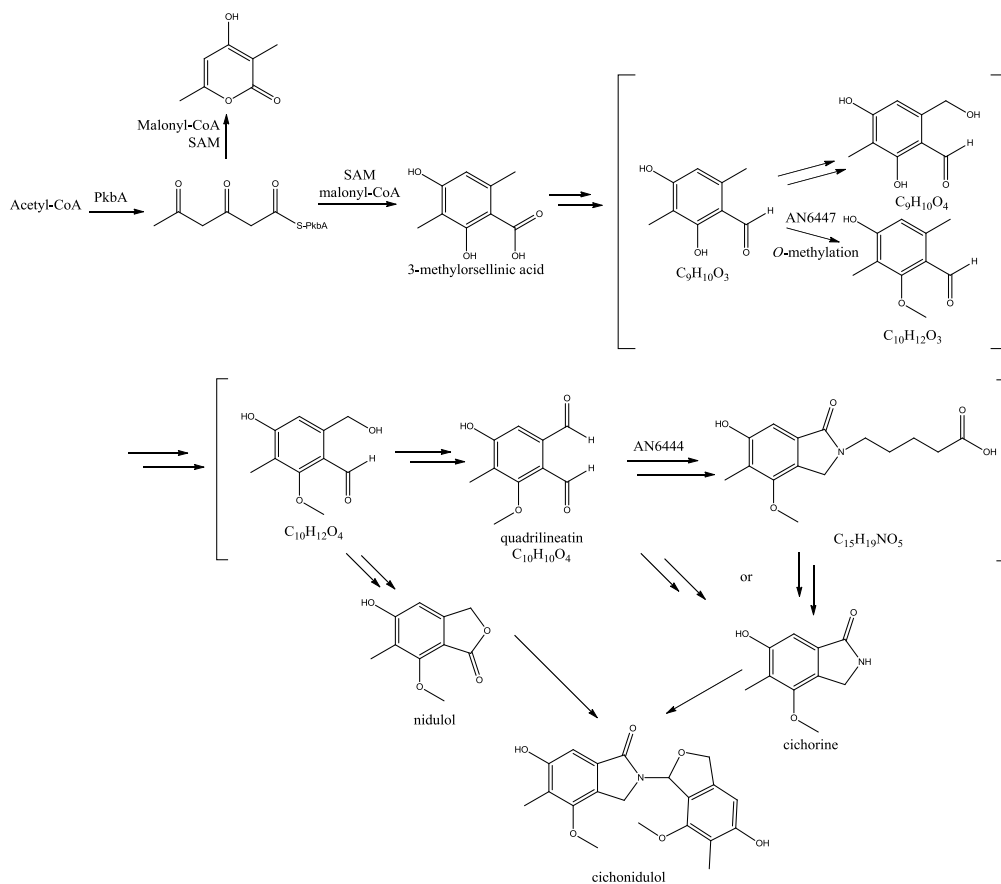
Figure 13 Proposed biosynthetic route of the elucidated metabolites of the pkbA cluster. The metabolites in boxes have all been identified through NMR-analyses, whereas the metabolites in brackets are proposed intermediates which have been detected through MS-analysis and the rest have not been detected.
