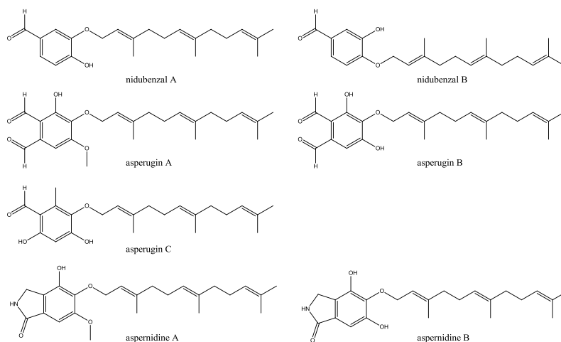
Figure 4.35 Structures of nidubenzal A and B ( 1 ), asperugin A, B ( 2 ), and C, and aspermidine A and B
