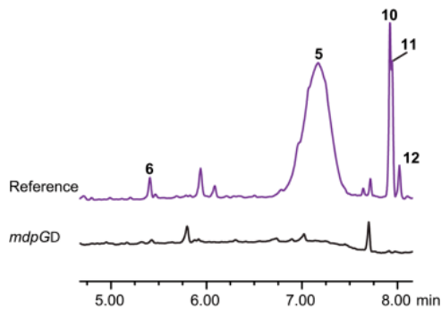
Fig. 2. The late portion of the UV-chromatogram (210 nm) of the Aspergillus nidulans reference strain and mdpGD on RTO medium. The deletion abolishes formation of arugosin A (5), arugosin H (6), emericellin (10), shamixanthone (11) and epi-shamixanthone (12) and a few unidentified peaks.
