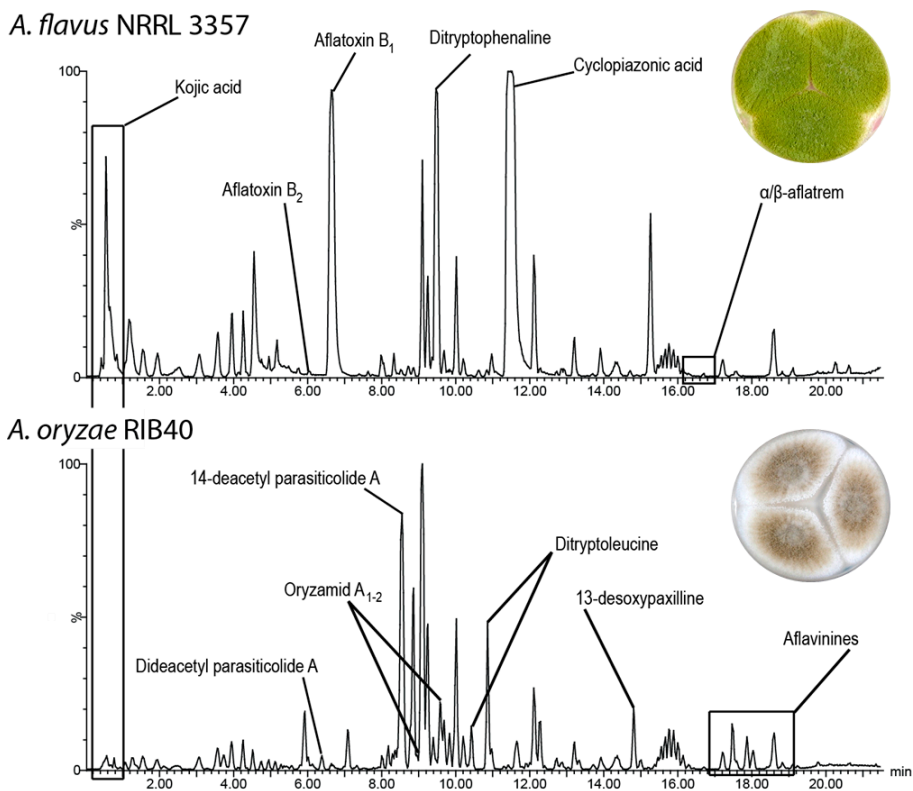
Figure 4.2 ESI+ (electrospray ionization) BPC (base peak chromatogram) of micro scale extract from WATM after seven days of incubation, bottom: A. oryzae RIB40, top: A. flavus NRRL3357. Besides kojic acid (shown in box) and analogues in the beginning of the chromatograms and ergosterol in the end (not shown), there are very few identical compounds between the genetically almost identical strains. Note that aspirochlorine is only detectable in negative ionization mode, and therefore not visible in these chromatograms. The oryzamides, dityryptoleucines and the parasiticolides are reported here. (figure taken from paper 2).
