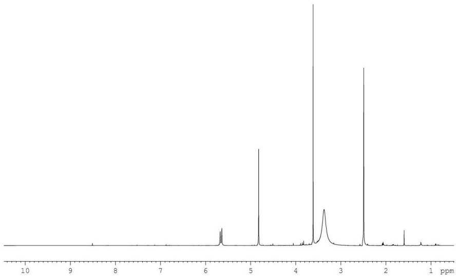
^1\text{H} NMR spectrum demethylnidulol in \text{DMSO-}d_6
