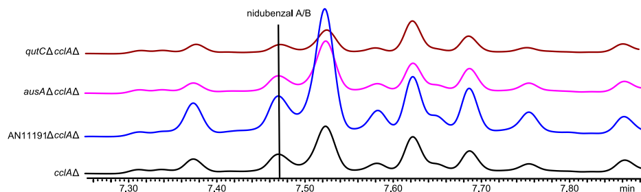
Figure 4.42 UHPLC chromatograms (210 nm) of micro-extracts of the qutC \Delta cclA \Delta , ausA \Delta cclA \Delta , AN11191 \Delta cclA \Delta and cclA \Delta strains after cultivation for seven days at 37°C on CY20 medium. The other parts of the chromatogram were also identical.
